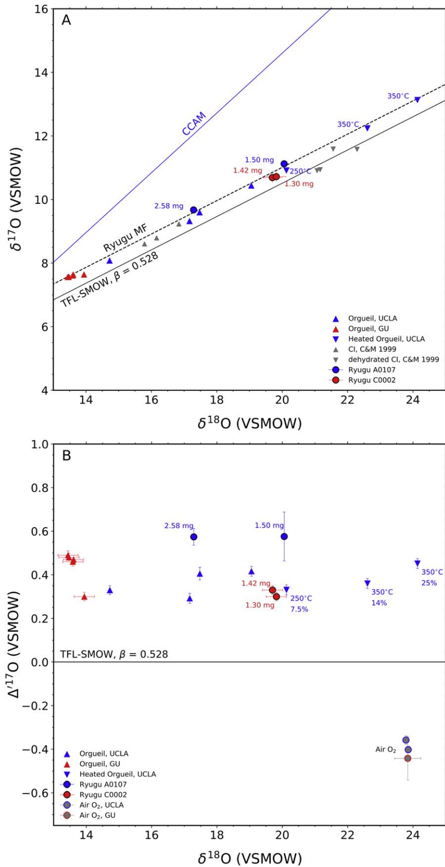
Figure 1. (a) Oxygen three-isotope plot comparing Ryugu milligram-sized samples (circles) with Orgueil meteorite values from this study and from the literature (triangles). (b) Plot of \Delta^{17}\text{O} vs. \delta^{18}\text{O} showing the results of Ryugu samples together with Orgueil meteorites (unheated vs. heated; heating temperature and mass-loss fraction are labeled in blue) and geostandards. “Ryugu MF” denotes the Ryugu mass-dependent fractionation curve (black dashed line) with \beta = 0.528 ; C&M refers to Clayton & Mayeda (1999).
