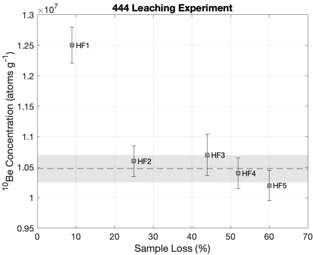
Figure 2. 10 Be concentrations measured after each of the five progressive leaches on pyroxenes from sample 444. Total sample material loss ranges from 9 % in Leach 1 to 60 % in Leach 5. The dashed black line shows the average 10 Be concentration of HF2–HF5, and the shaded box shows the standard deviation of those 10 Be concentrations. The HF2–HF5 concentrations overlap within uncertainty, suggesting that 20 %–25 % sample loss is enough to sufficiently remove meteoric 10 Be from old Ferrar dolerite samples.
