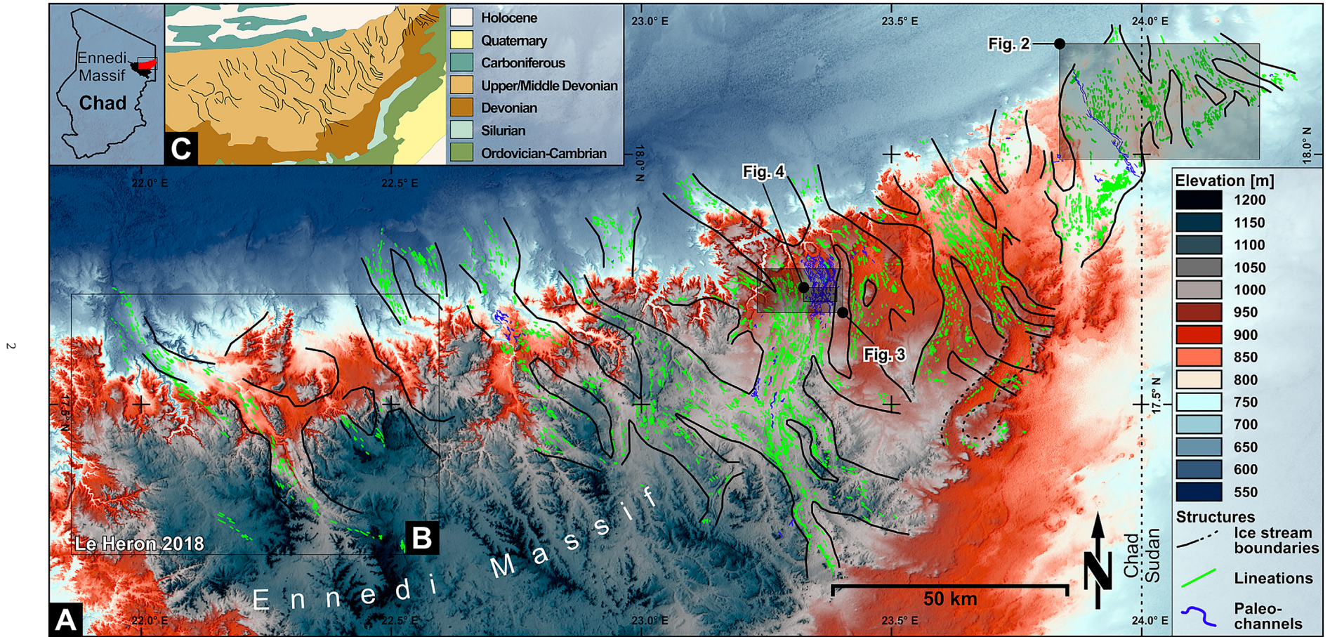
Fig. 1. False colour image based on Shuttle Radar Topography Mission (SRTM-1 Arcsec) of the Ennedi Plateau with mapped glacial lineations (GLs) and ice stream boundaries developed on Devonian deposits (A), inset images correspond to Figs. 2, 3 and 4 . Area mapped in this paper shown next to the area mapped in Le Heron (2018) (B). (C) Geology after Persits et al. (1997) .
