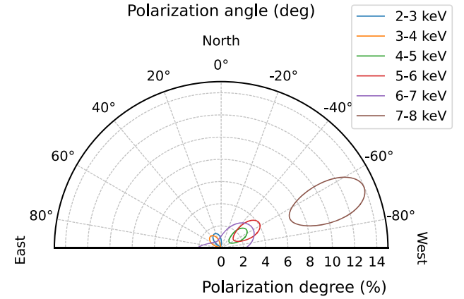
Figure 6. Top: normalized Stokes parameters Q/I and U/I in different energy bins as measured with PCUBE in IXPEOBSSIM. Bottom: polar plot of the X-ray polarization in 4U 1820–303 when 1 keV binning is applied. Contours are reported at 68% CL. A trend of polarization growing with energy is visible in both plots.
