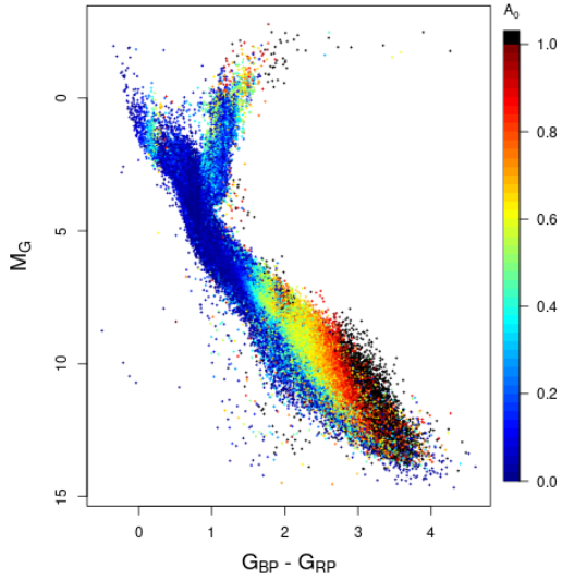
Fig. 30. Hertzsprung-Russell diagram of low-extinction stars ( A_0 < 0.05 mag according to Lallement et al. 2019) with a parallax relative precision lower than 10%, colour-coded with the mean extinction a_{\text{zero\_gspphot}} . The colour is saturated as black for values higher than 1 mag. In this low extinction sample, M_G is simply G + 5 + 5 \log(\varpi/1000) .
