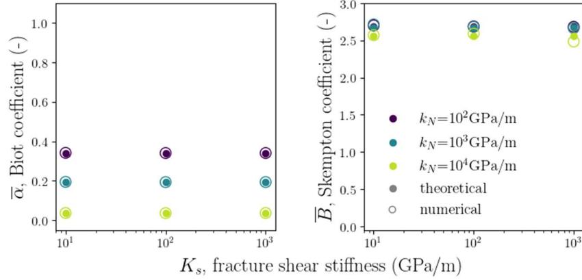
Figure 7. Comparison between theoretically (full markers) and numerically (empty markers) estimated equivalent Biot and Skempton coefficients, for a non-porous rock hosting parallel infinite fractures crossing with an angle of 40^\circ , and for different values of fracture normal and shear stiffness, \kappa_N and \kappa_s . The case of loading in x -direction is shown.
