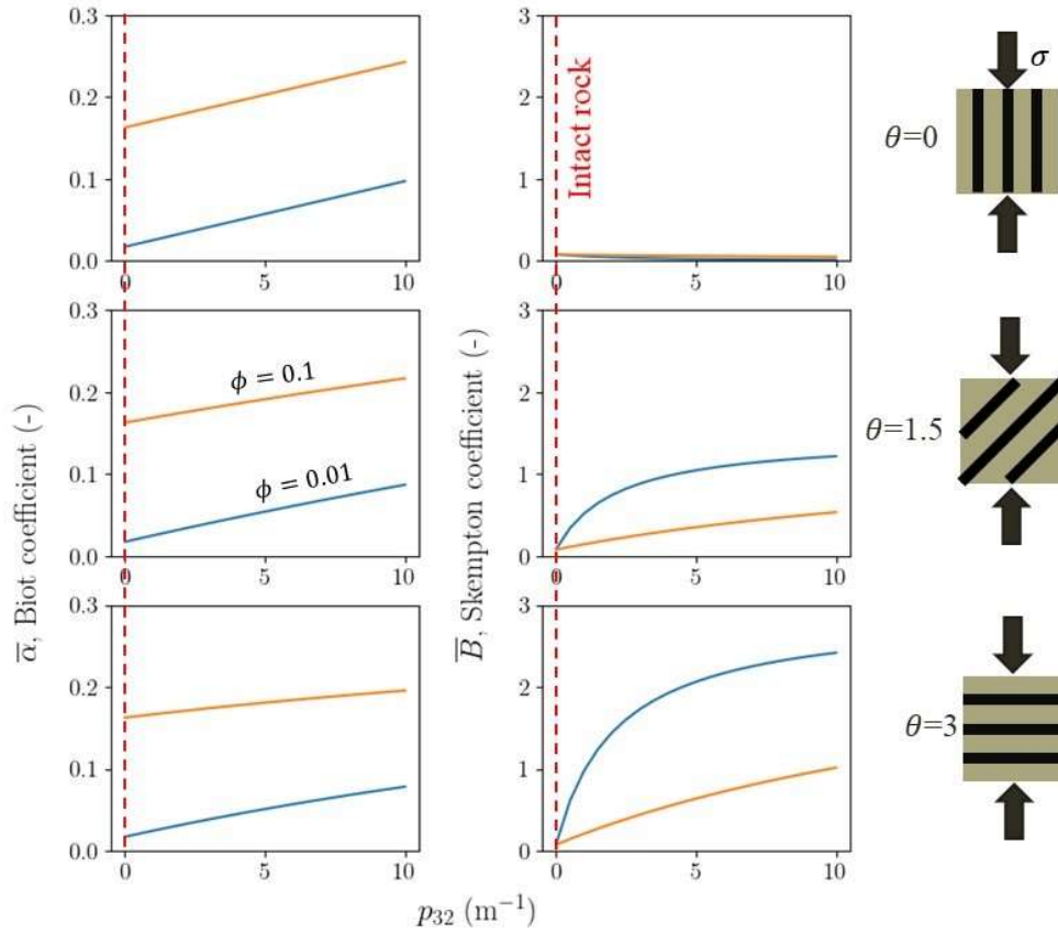
Figure 8. Sensitivity of the equivalent Biot and Skempton coefficients to fracture density ( p_{32} ) and to intact rock porosity ( \phi ). The analysis considers a vertical load applied to a porous rock, with E=60 GPa and \nu=0.25 , hosting a set of parallel fractures with equal e=10\mu\text{m} , \kappa_N=5000 GPa/m, and orientation, for which three values of \theta are analyzed. Colors refer to different values of \phi . The red dashed vertical line defines the case with p_{32}=0 , corresponding to intact rock with no fractures.
