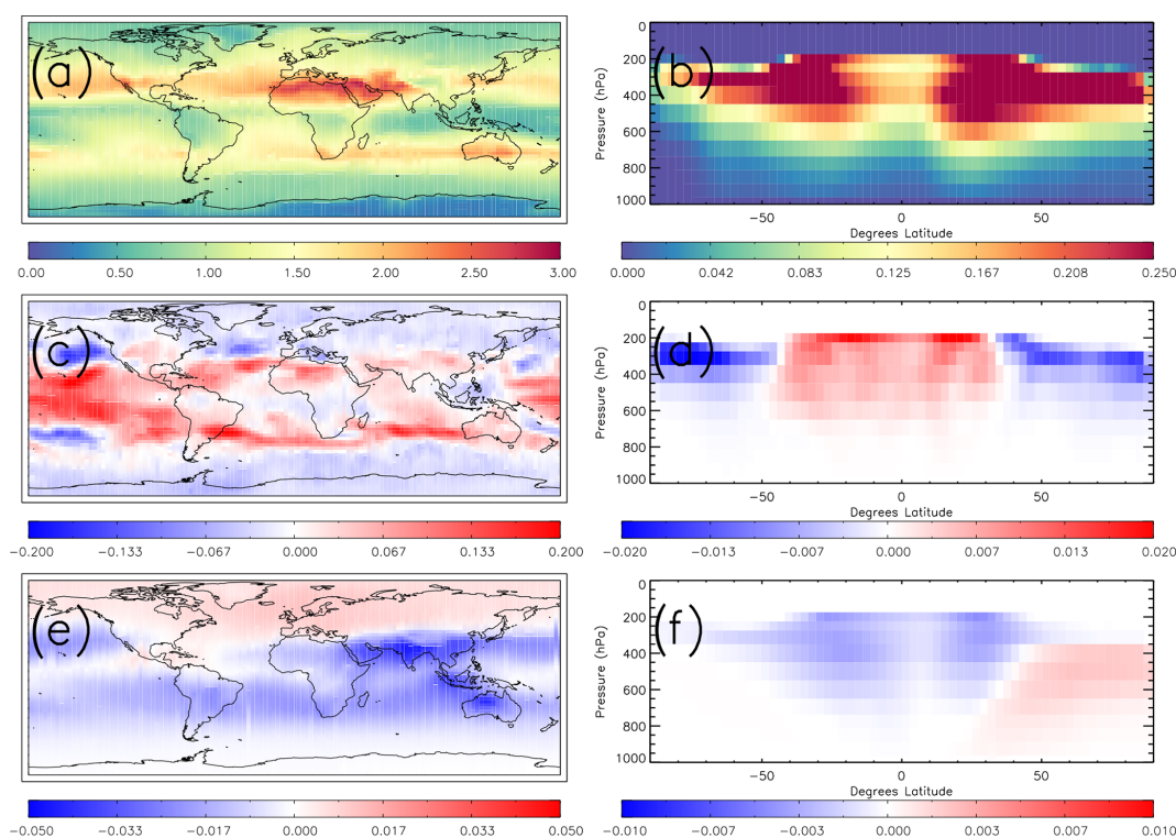
Figure 4. (a) TOMCAT control run \text{TO}_3\text{RE} ( \text{W m}^{-2} ), (b) TOMCAT control run zonal average grid box \text{O}_3 radiative effect ( \text{W m}^{-2} ), (c) TOMCAT fixed meteorology–TOMCAT control \text{TO}_3\text{RE} difference ( \text{W m}^{-2} ), (d) TOMCAT fixed meteorology–TOMCAT control zonal average grid box \text{O}_3 radiative effect difference ( \text{W m}^{-2} ), (e) TOMCAT fixed emissions–TOMCAT control \text{TO}_3\text{RE} difference ( \text{W m}^{-2} ), and (f) TOMCAT fixed emissions–TOMCAT control zonal average grid box \text{O}_3 radiative effect difference ( \text{W m}^{-2} ).
