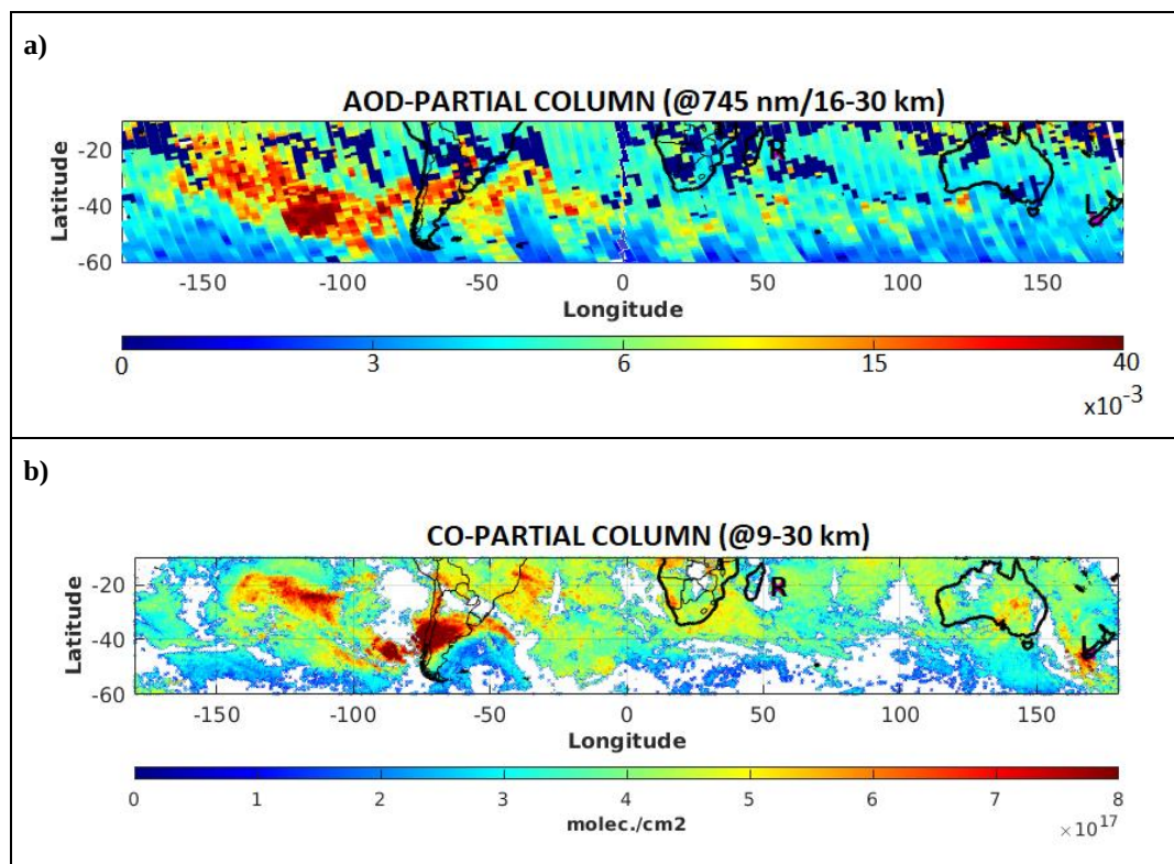
Figure 4: Time-averaged map (from 9 th to 16 th January 2020) of (a) sAOD (between 16 and 30 km at 745 nm) obtained from OMPS observations and (b) partial column of CO (averaged between 9 and 30 km) obtained from IASI observations. The location of Reunion and Lauder sites are indicated by R and L respectively.
