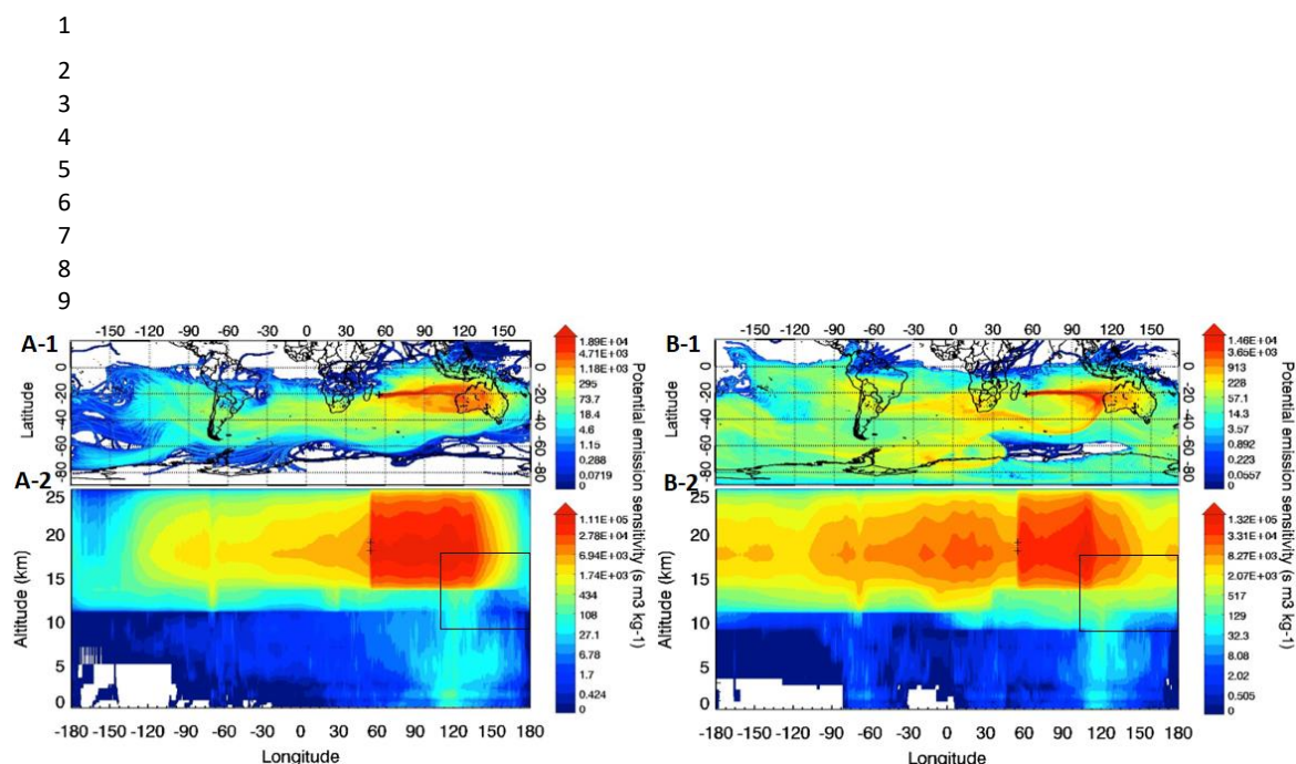
Figure 7: FLEXPART 30-day back trajectories initialized from Reunion (black cross) at 18 km on 27 th January 2020 (A-1-2) and 28 th January 2020 (B-1-2). A-1 and B-1 correspond to an integration of the trajectory positions over the whole altitude range. A-2 and B-2 are the vertical view integrated over the whole latitude range of the back trajectories A-1 and B-1. The black rectangle represented the injection height of the biomass burning aerosols.
