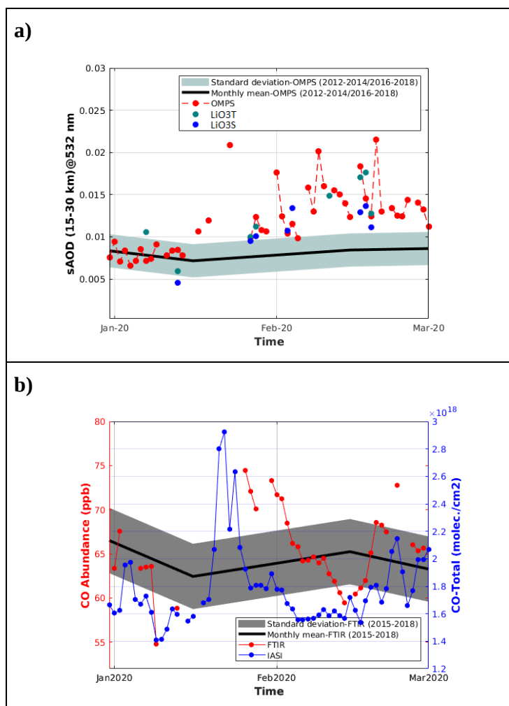
Figure 5: Daily mean evolution of aerosol (a) and CO (b) abundances obtained from ground-based and satellite observations at Reunion between 1 st January and 1 st March 2020. Total column (molecule.cm -2 ) and abundance (ppb) of CO obtained from IASI (blue line) and FTIR (red line) respectively are given in the lower panel (b), while sAOD obtained from OMPS (red line) and Lidar (blue and green dots) are given in the upper panel (a). The black and dashed lines correspond to monthly mean and the associated standard deviation calculated during the background period.
