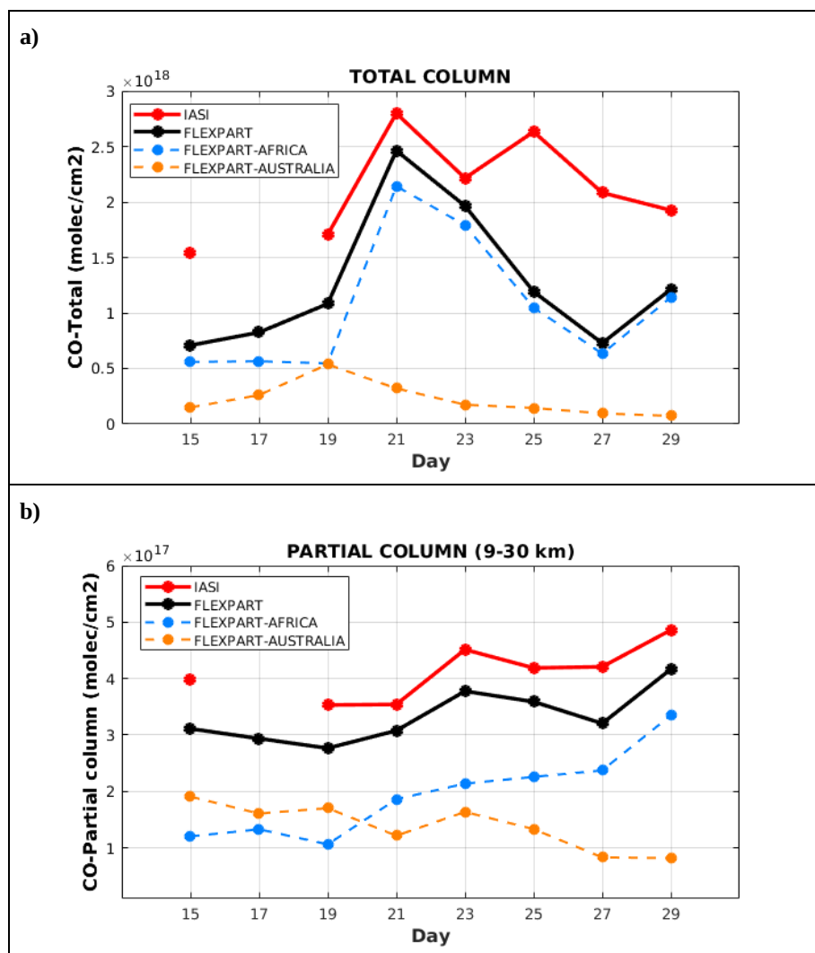
Figure 12: Daily evolution of (a) total column and (b) partial column (calculated between 9 and 30 km) of CO observed by IASI (red line) and simulated by FLEXPART (black line) over Reunion from 15 th to 29 th January 2020. The CO evolution is simulated by FLEXPART in considering only the CO emission (including BB and anthropogenic activity) from African (cyan line) and Australian (orange line) BB sources.
