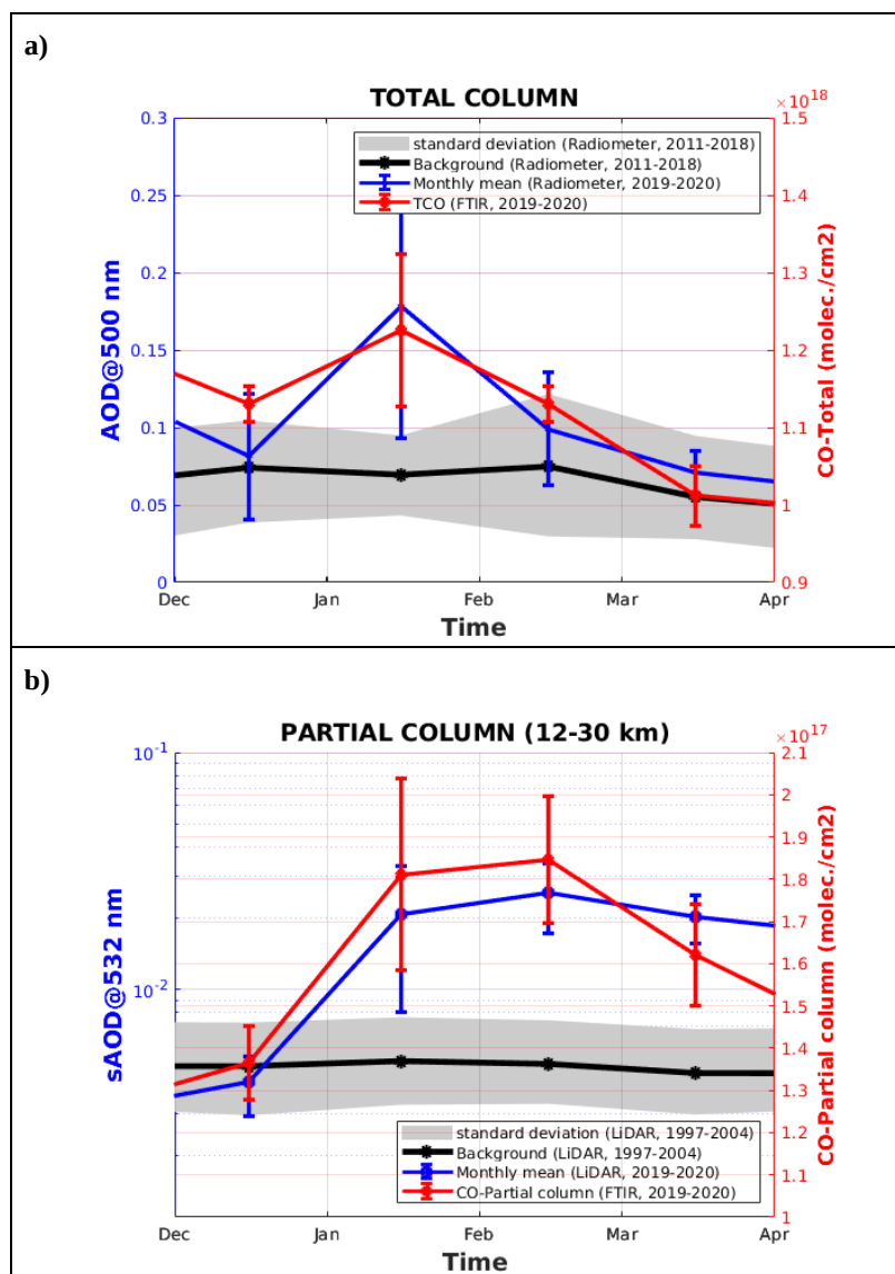
Figure 3: (a) Monthly mean evolution of total column of aerosol (AOD at 500 nm) and CO obtained from SKYNET radiometer and FTIR respectively over Lauder from 1 st December 2019 to 1 st April 2020. (b) Monthly mean evolution of the stratospheric AOD (sAOD) and CO (sCO) columns at Lauder between 1 st December 2019 and 1 st April 2020. The sAOD and sCO are calculated between 12 and 30 km from lidar and FTIR measurements respectively. The background evolution of aerosol data (AOD: 2011-2018 and sAOD: 1997-2004) and the associated standard deviation are given in black lines and grey areas, respectively.
