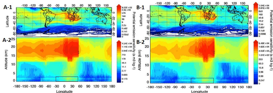
Figure 9: Same as figure 7 with an injection height initialized at 16 km.
