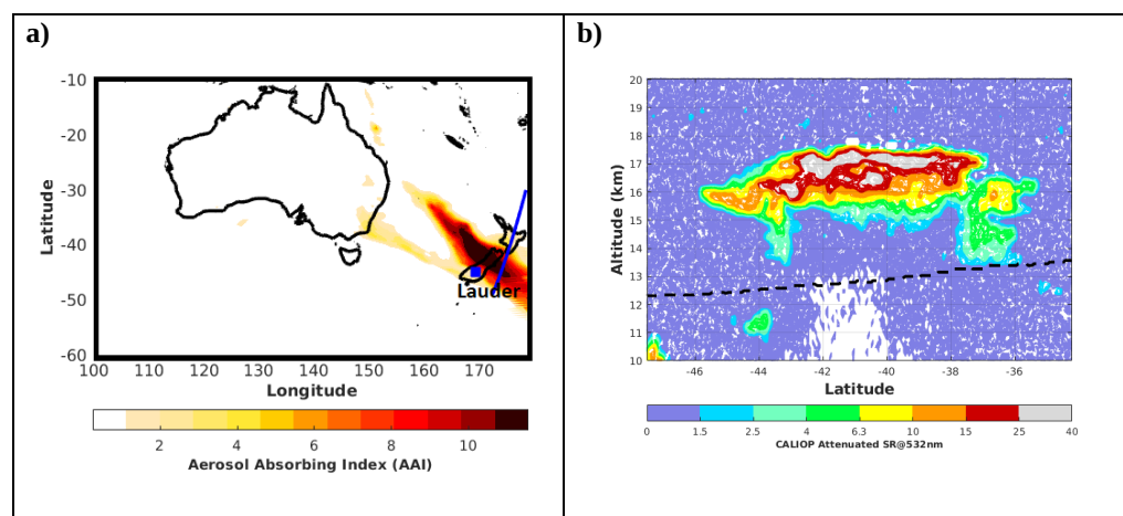
Figure 1: (a) Map of Aerosol Absorbing Index obtained from OMPS observations and (b) scattering ratio profiles at 532 nm obtained from CALIOP observations on 1 st January 2020. The orbit overpass of CALIOP is indicated by the blue curve, while the blue square corresponds to the Lauder site in plot (a). The black dashed line in (b) corresponds to the 380 K isentropic level calculated from CALIOP observations.
