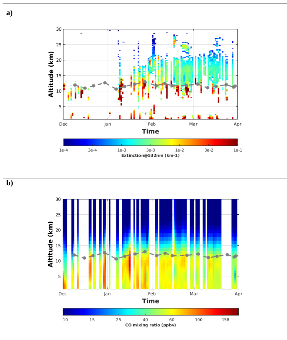
Figure 2: Time series of daily profiles at Lauder of (a) aerosol extinction at 532 nm obtained from lidar and (b) CO mixing ratio obtained from FTIR between 1 st December 2019 and 1 st April 2020. In order to screen non-aerosol contributors (such as clouds) on the extinction measurements, a mask based on the method reported by Nicolae et al. (2013) that includes consideration on plausible aerosols properties was used. Namely, we only kept profile parts with positive depolarization values, and Angström exponent ranges from 0.1 to 4. The grey line indicates the tropopause height obtained from radiosonde measurements.
