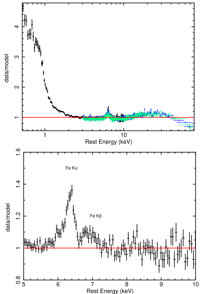
Figure 1. Upper: Broad-band (0.3–79 keV) residuals when the main continuum is fitted in the 3–5 and 7.5–10 spectral regions. The black spectrum represents the EPIC-pn data, FPMA and FPMB data are shown in the same colour, blue for Epoch 1 and green for Epoch 2. Lower: Zoom on the 5–10 keV spectral region, with XMM-Newton (EPIC-pn, black) as a ratio to an absorbed power law with a photon index \Gamma = 1.86 and a column density N_{\text{H}} = 1.6 \times 10^{22} \text{ cm}^{-2} .
