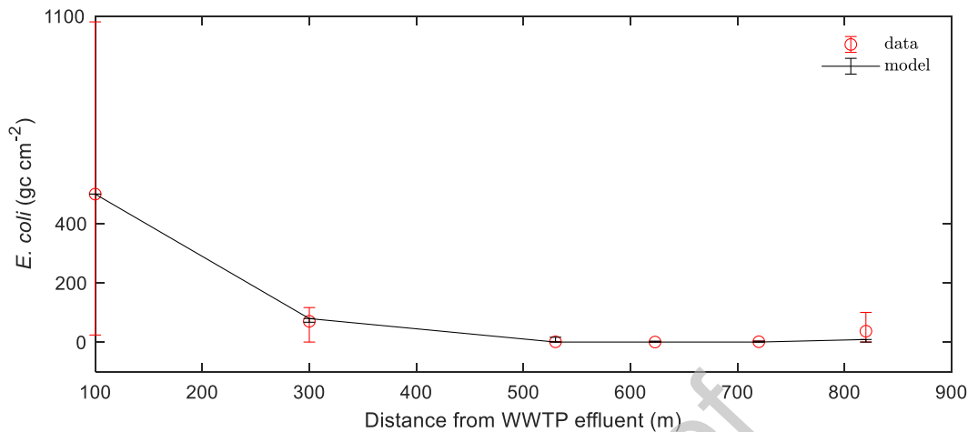
Figure 2. Data vs model at sampling sites 100 - 820 m downstream of a WWTP effluent point source during baseflow conditions (July). Best-fit parameters shown in Table 2.
