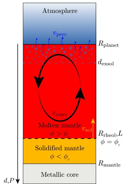
Fig. 10 Schematic of the magma ocean degassing process and associated velocities. v_{sol} is the upward solidification velocity associated with the uprising rheological front where \phi = \phi_c (assuming that solidification proceeds from bottom-up). v_{conv} is the liquid-like convection velocity and v_{perc} is the percolation velocity of the gas bubbles rising up to the surface. d_{exsol} is the exsolution depth above which oversaturated volatiles are exsolved out of the melt and start forming gas bubbles. In a rapidly convecting magma ocean, volatile-bearing melt is assumed to reach the exsolution depth much faster than solidification proceeds and loses its volatiles in excess of saturation on that occasion. The outgassing is thus often assumed to be efficient. Adapted from Salvador and Samuel (2023)
