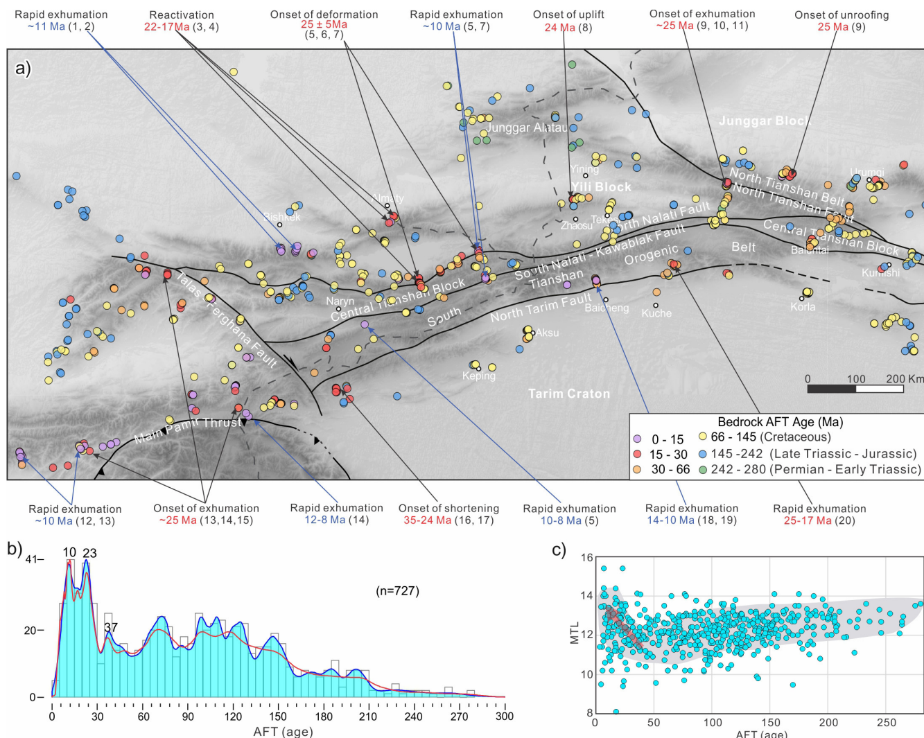
FIGURE 8: (a) Previously published basement AFT ages plotted on a Digital Elevation Model (DEM) of Chinese western Tianshan and Kyrgyz Tianshan (data sources in Supplementary Table S4), with major faults and Cenozoic tectonic events based on AFT data also depicted (1 [44]; 2 [102]; 3 [71]; 4 [70]; 5 [103]; 6 [104]; 7 [105]; 8 [106]; 9 [6]; 10 [107]; 11 [108]; 12 [109]; 13 [110]; 14 [111]; 15 [112]; 16 [113]; 17 [76]; 18 [21]; 19 [45]; 20 [114]). (b) AFT age spectra where blue lines and fill are Kernel density estimate curves, and the red lines are the probability density distribution. (c) “Boomerang plot” of AFT central age against MTL.
