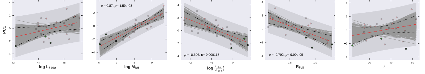
Fig. 14. Correlations between the first principal component (PC1) and the physical properties of the sample. From left to right: correlation with the AGN luminosity at 5100 Å ( L_{5100\text{Å}} , in units of \text{erg s}^{-1} ), the black hole mass ( M_{\text{BH}} , in units of M_{\odot} ), the Eddington ratio, the ratio R_{\text{FeII}} , and the viewing angle ( i ). Our three sources (Mrk 1044, SDSS J080101.41+184840.7, and, IRAS 04416+1215) are marked in green, while the other sources are marked in red. The Spearman's rank correlation coefficients ( \rho ) and the p -values are reported for the correlations whenever the p -value < 0.001 . The ordinary least-square fit for each panel is shown using a red solid line. The black dotted lines mark the confidence intervals at 95% for the 1000 realizations (dark gray lines) of the bootstrap analysis. The corresponding prediction intervals are shown in the background using a light gray color.
