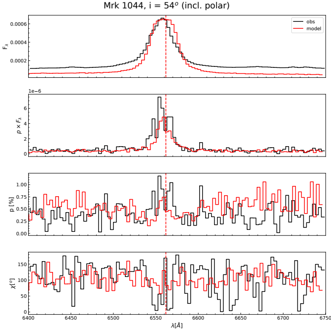
Fig. 6. STOKES modeling for Mrk 1044 with the equatorial plus polar scattering region and comparison with observational estimates. The case shown has a viewing angle of 54°. From top to bottom: spectrum in natural light ( F_\lambda ), polarized spectrum ( p \times F_\lambda ), polarization fraction ( p ), and polarization angle ( \chi ). The vertical red dashed line marks the central wavelength for H \alpha .
