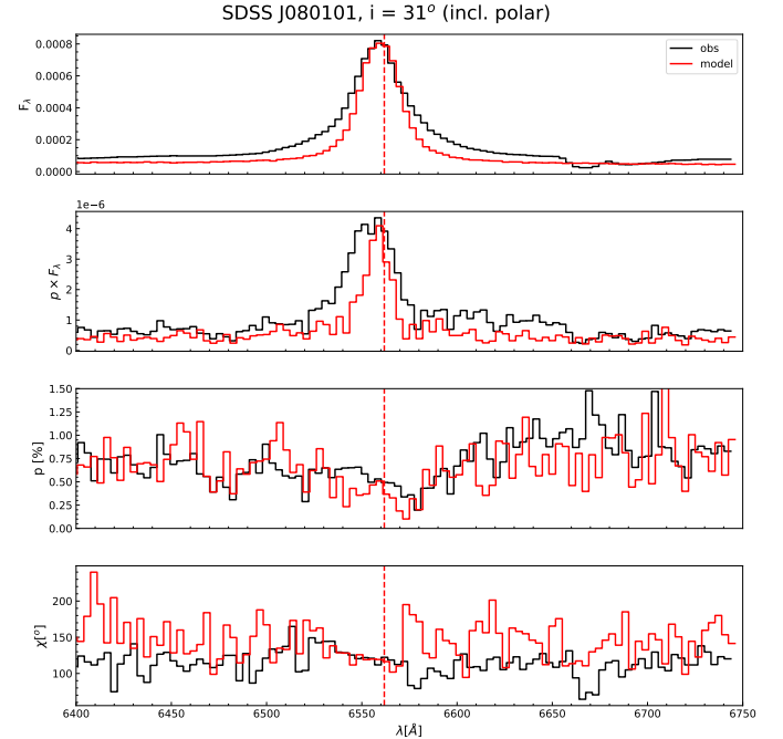
Fig. 7. STOKES modeling for SDSS J080101.41+184840.7 with the equatorial plus polar scattering region and comparison with observational estimates. The case shown has a viewing angle of 31°. The panels depict the same parameters as described in Fig. 6.
