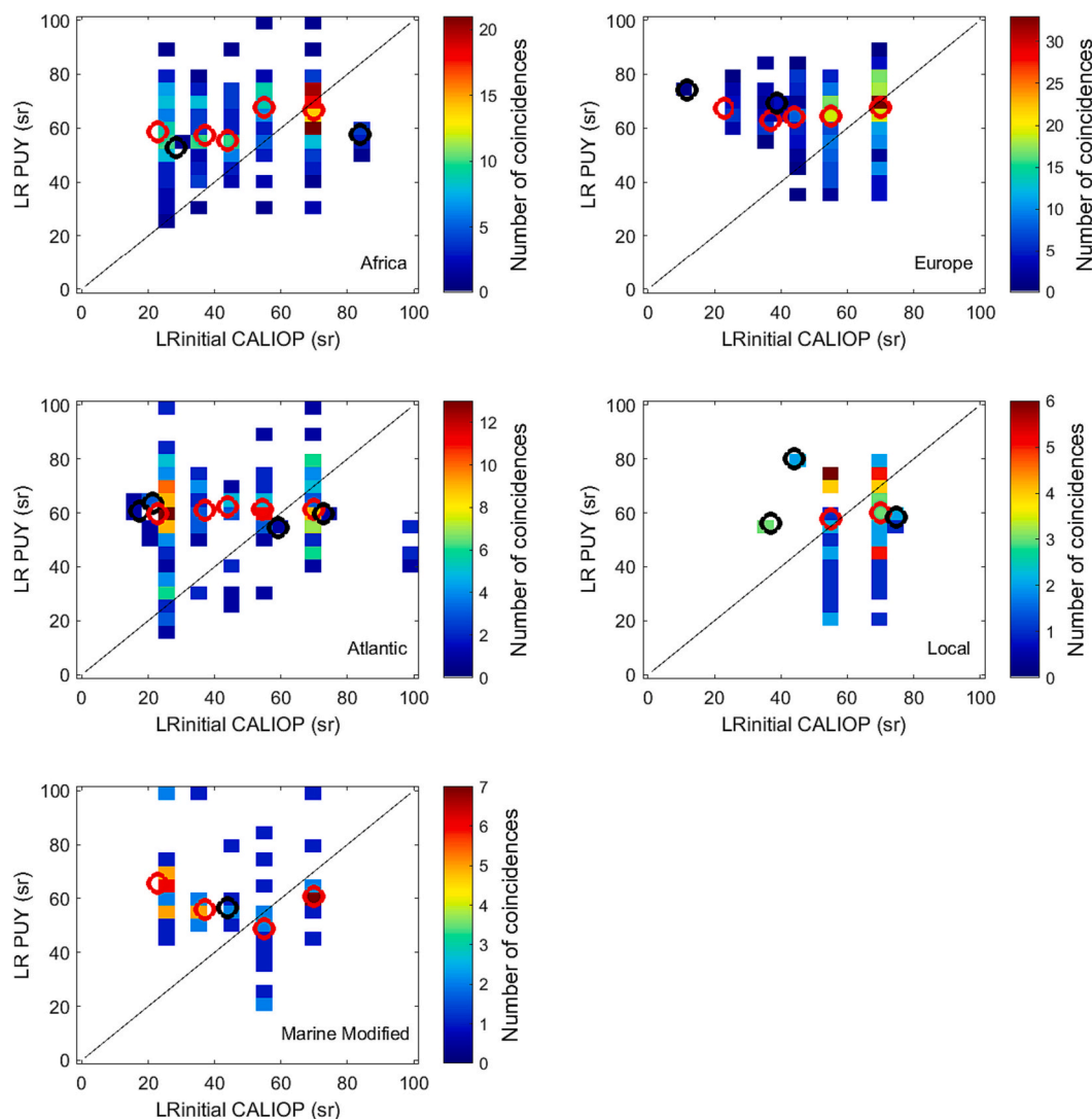
Fig. 7. Density plot of the LR for the coincidences founded between CALIOP (x-axis) and the backtrajectories calculated from PUY observations (y-axis) by bins of 5 sr for each sector indicated on the graph. For each CALIOP discrete value, the median of the LR PUY has been calculated and shown by a circle in black when there is <10 LR and in red when there is >10 LR.
