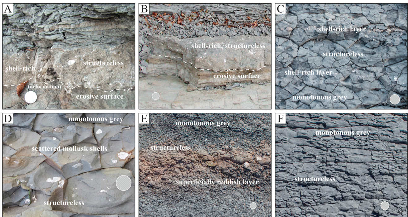
Fig. 11. Common features of the lake-dominated facies association. A, B. Typical thin sandstones (shoreface) interfingering with shallow delta facies association. C-F. Typical muds (offshore).
