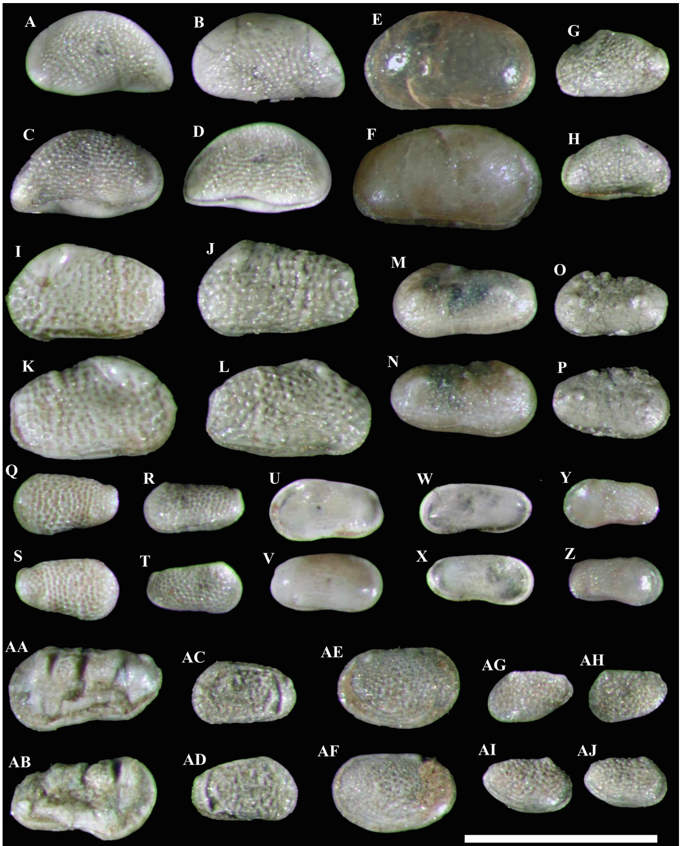
Fig. 9. Common ostracods from the Pontian in the Slănic de Buzău section. A–D. Bakunella dorsoarcurata (Zalányi, 1929). E, F. Cyprideis ex. gr. torosa (Jones, 1850). G, H. Pontoleberis pontica (Stancheva, 1965). I–L. Tyrrhenocythere filipes (Hanganu, 1962). M, N. Cytherissa bogatschovi Livalent, 1929. O, P. Cytherissa ex. gr. bogatschovi (Livalent, 1929). Q–T. Amnicythere andrusovi (Livalent, 1929). U, V. Euxinocythere cornutocostata (Schweyer, 1949). W, X. Amnicythere cymbula (Livalent, 1929). Y, Z. Amnicythere sinigubi (Krstić, 1975). AA, AB. Amnicythere multituberculata (Livalent, 1929). AC, AD. Maeotocythere ex. gr. bosqueti (Livalent, 1929). AE, AF. Loxoconcha petasa Livalent, 1929. AG–AJ. Loxoconcha babazanonica Livalent, 1929. Scale bar: 1 mm.
