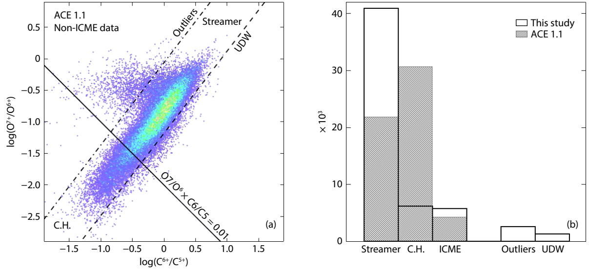
Figure 3. (a) 2D histogram of the \log(\frac{O^{7+}}{O^{6+}}) versus the \log(\frac{C^{6+}}{C^{5+}}) ratio from the non-ICME (Interplanetary Coronal Mass Ejection) ACE SWICS 1.1 data. The black lines represent the coronal hole — streamer (solid), the outlier (dot-dashed) and the Upper Depleted Wind (UDW) (dashed) type separation (see text for details). (b) Comparison of the solar wind type histogram for this analysis and the ACE 1.1 website classification.
