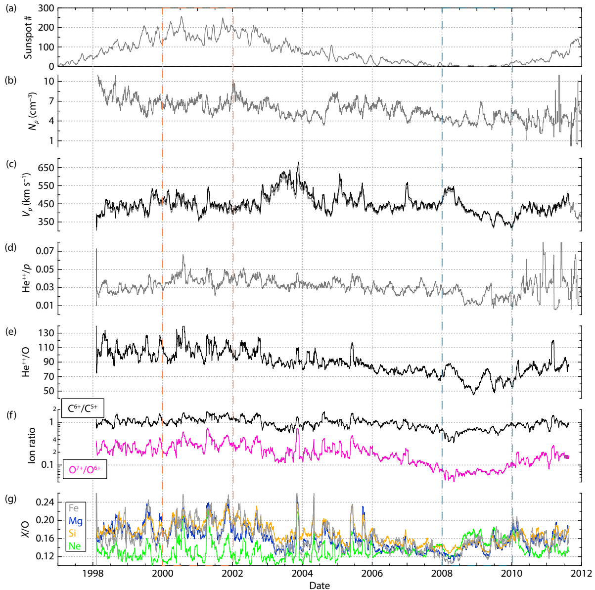
Figure 2. From top to bottom: (a) Sunspot number, (b) Proton density from SWEPM, (c) Proton (grey) and alpha particle (black) velocities from SWEPM and SWICS respectively, (d) alpha to proton ratio from SWEPM, (e) alpha to oxygen ratio from SWICS, (f) Carbon (black) and Oxygen (magenta) charge state ratios, (g) Elemental abundances of the heavy ions measured with SWICS (Neon–green, Magnesium–blue, Silicon–yellow, Iron–grey). All quantities are 27-day averages. The orange and blue dashed rectangles mark out respectively the solar maximum and solar minimum limits applied in calculations (See text for details).
