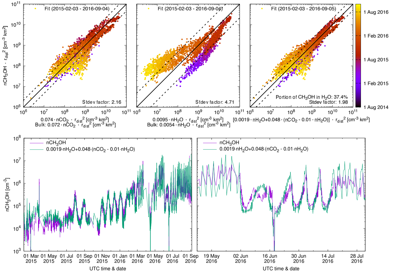
Figure 6. Same as Fig. 4 but for CH 3 OH instead of CH 4 .
