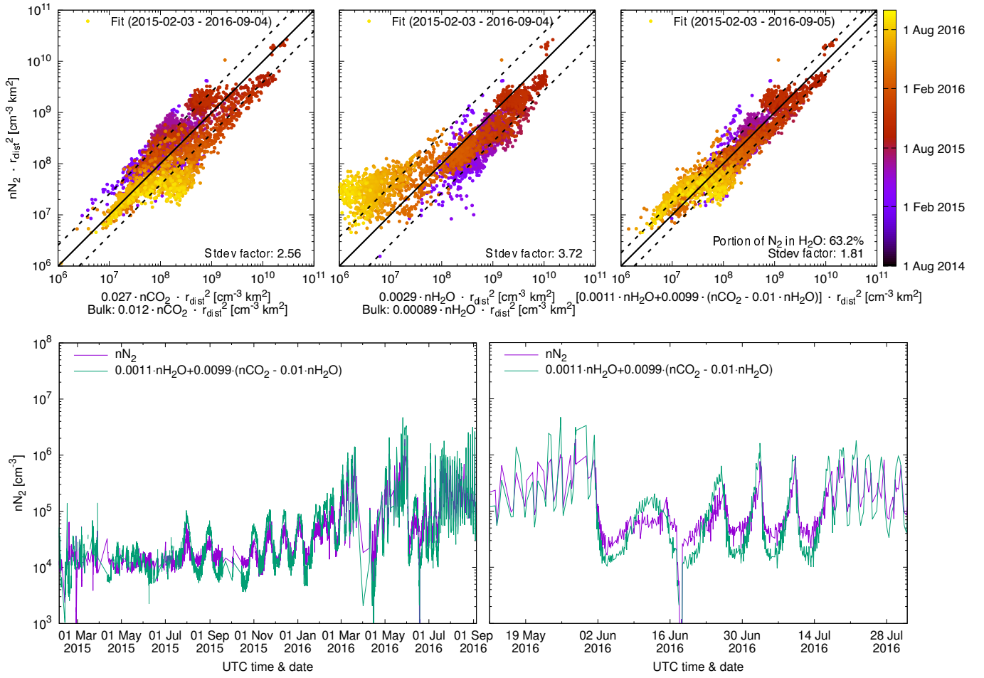
Figure B2. Same as Fig. 4 but for \text{N}_2 instead of \text{CH}_4 .
