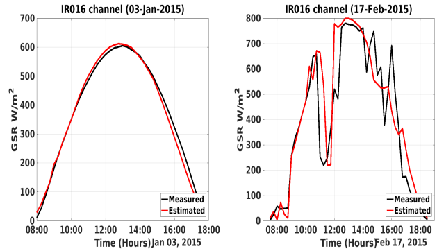
Fig. 5: Estimated GSRGL (red) superimposed on that measured (black) in a clear (left) and a cloudy (right) day.
