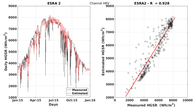
Fig. 2: Left: Daily variations of the cumulative HGSI estimated with HRV images (red) and from measurements (black). Right: Linear regression between the two quantities.
