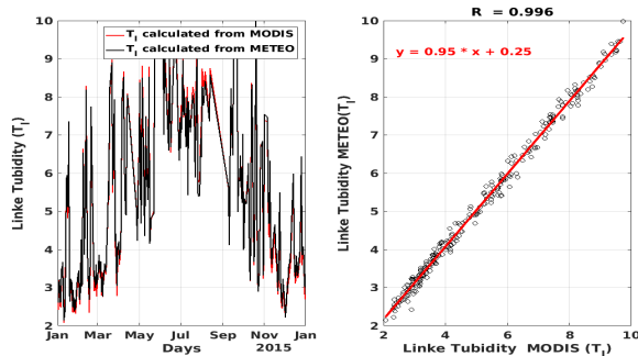
Fig. 1: Left: Temporal variation of T_l estimated from water vapor data obtained from MODIS (red line) and from meteorological measurements made in Ghardaïa (black line). Right: good correlation between the two T_l datasets.
