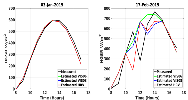
Fig. 3: Estimated GSRGL (red) superimposed on that measured (black) in a clear (left) and a cloudy (right) day.
