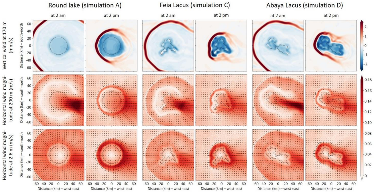
Figure 8. Maps, at 2 am and 2 pm, of vertical wind at 170 m and horizontal wind at 200 m and 2.6 m. Comparison of circulations obtained with a round lake (simulation A), Feia Lacus (simulation C) and Abaya Lacus (simulation D), with background wind. The black dashed lines indicate the position of the lake. The arrows indicate the direction and relative intensity of the horizontal wind.
