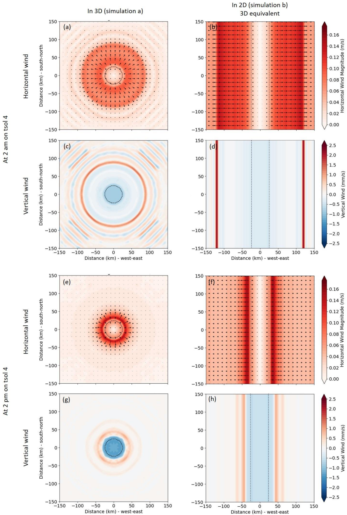
Figure 3. Maps of horizontal (at 2.6 m) and vertical (at 170 m) winds at 2 am and 2 pm local time. Comparison of atmospheric circulations obtained in 3D (simulation a) and 2D (simulation b) for a 50 km diameter lake. In the 2D case, the equivalent 3D map is plotted, with a lake infinitely long along the y-axis. The black dashed lines indicate the position of the lake. The arrows indicate the direction and relative intensity of the horizontal wind at 2.6 m.
