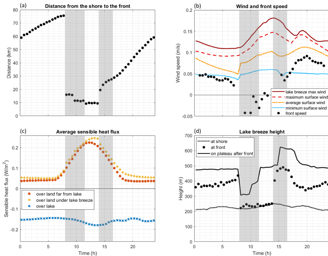
Figure 13. Comparison of the characteristics of the lake breeze in the reference simulation [a]. (a) Distance from the shore to the front, (b) characteristic winds and front speed, (c) sensible heat flux, and (d) lake breeze characteristic heights. The lake breeze maximum wind is the maximum horizontal wind in the total volume of the lake breeze. The average surface wind is the average of the horizontal wind magnitude in the surface area covered by the lake breeze at the first level (2.6 m). Grey zones indicate times when the front is more diffuse.
