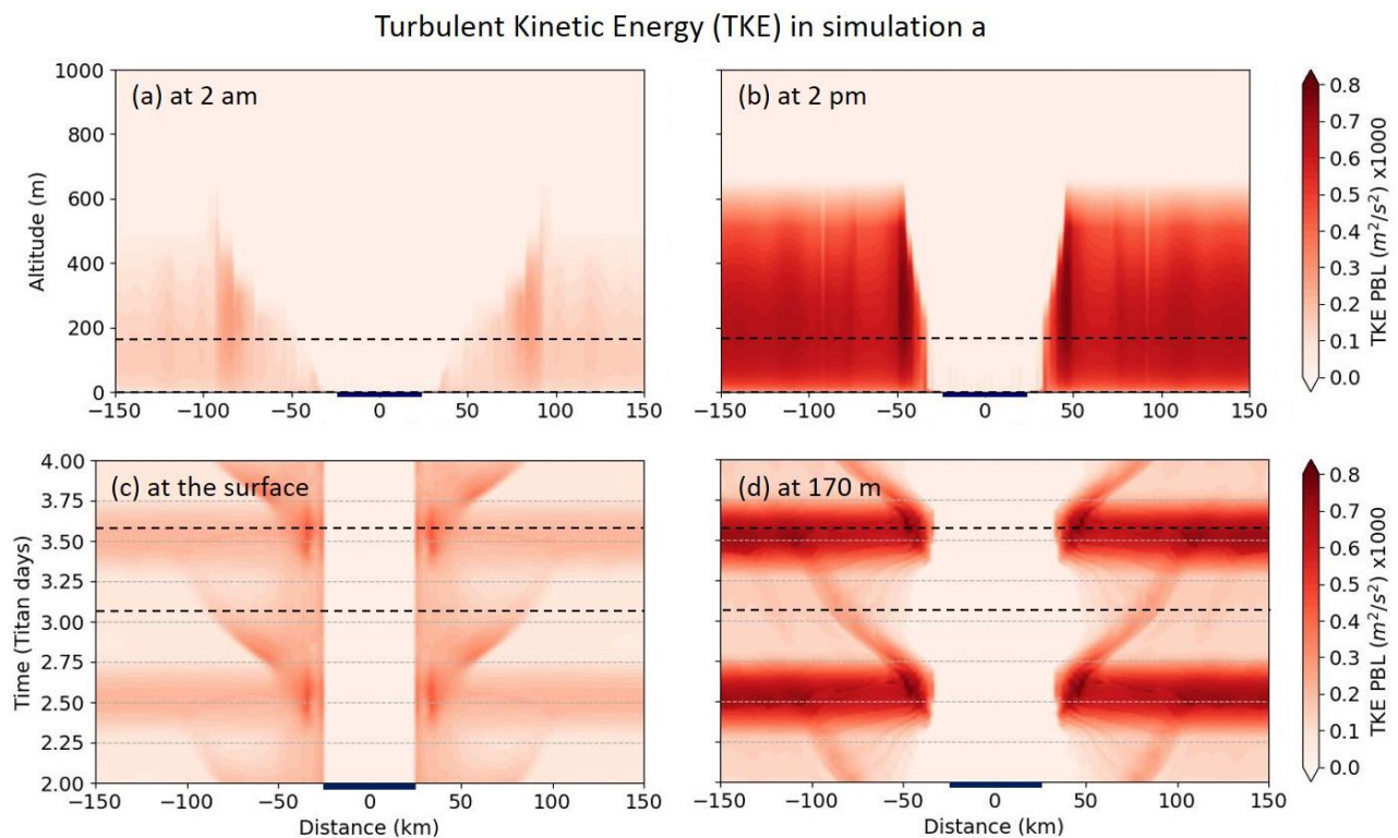
Figure A1. Turbulent Kinetic Energy (TKE) as function of altitude and time for a round lake of 50 km without background wind (simulation a). The dark blue bars below the plots indicate the position of the lake. The black dashed lines indicate the position of the slices plotted with different axes.
