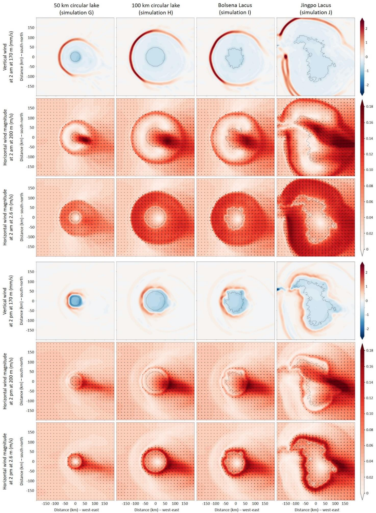
Figure 11. Maps, at 2 am and 2 pm, of vertical wind at 170 m and horizontal wind at 200 m and 2.6 m. Comparison of circulations obtained with a 50 km circular lake (simulation G), a 100 km circular lake (simulation H), Bolsena Lacus (simulation I) and Jingpo Lacus (simulation J) with a background wind. The black dashed line indicates the position of the lake. The arrows indicate the direction and relative intensity of the horizontal wind.
