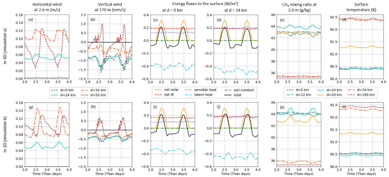
Figure 4. Evolution with time of surface horizontal wind, vertical wind at 170 m, energy fluxes over the lake, methane mixing ratio and surface temperature. Comparison of results obtained in 3D (simulation a) and 2D (simulation b) for a 50 km lake. The parameter d is the distance to the center of the lake. Energy fluxes are defined from the atmosphere (or from the subsurface) to the surface so that positive fluxes participate to heat the surface, and negative fluxes to cool the surface.
