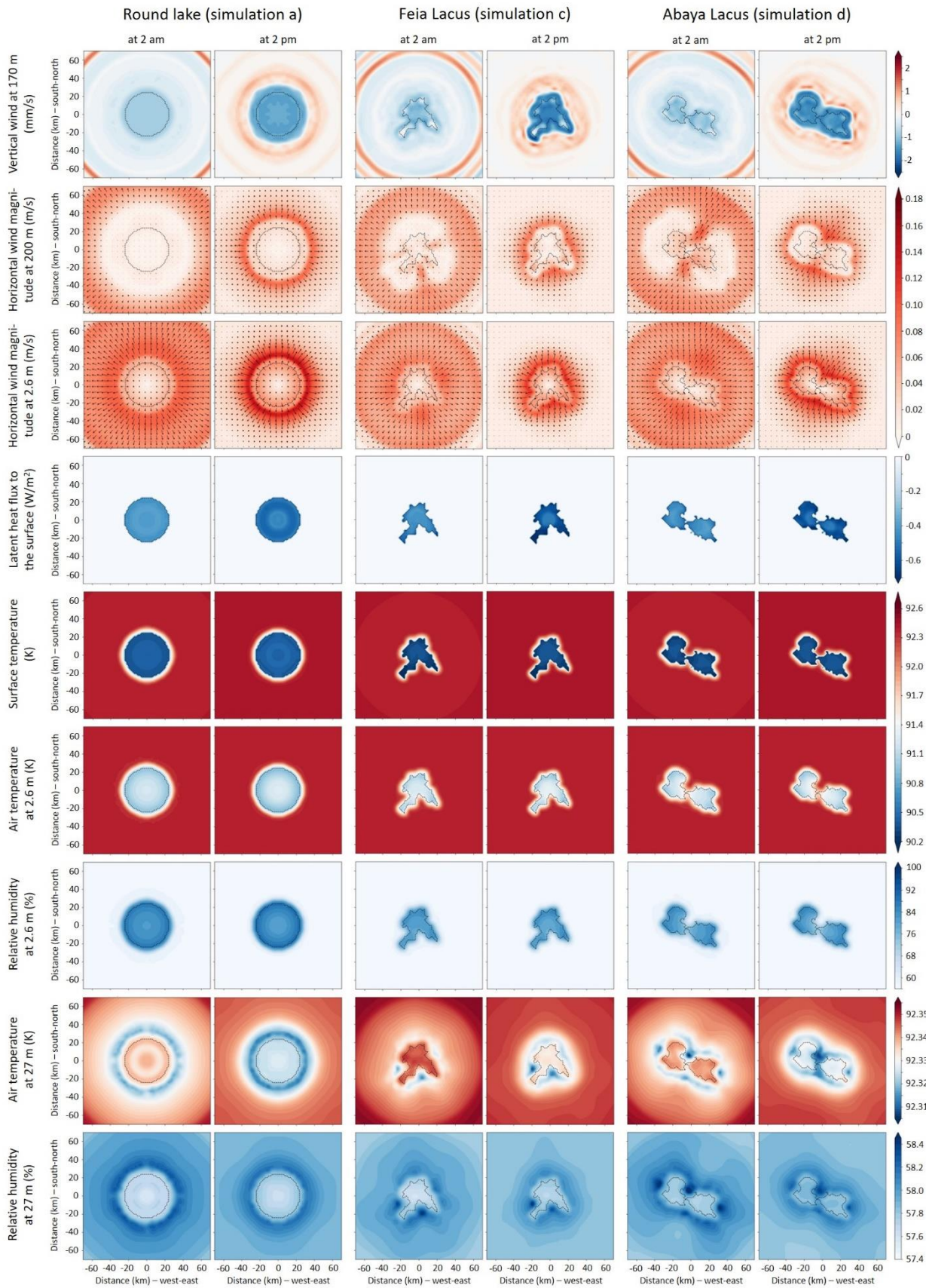
Figure 7. Maps, at 2 am and 2 pm, of vertical wind at 170 m, horizontal wind at 200 m and 2.6 m, latent heat flux to the surface, surface temperature, and air temperature and relative humidity at 2.6 m and 27 m. Comparison of circulations obtained with a round lake (simulation a), Feia Lacus (simulation c) and Abaya Lacus (simulation d). The black dashed lines indicate the position of the lake. The arrows indicate the direction and relative intensity of the horizontal wind.
