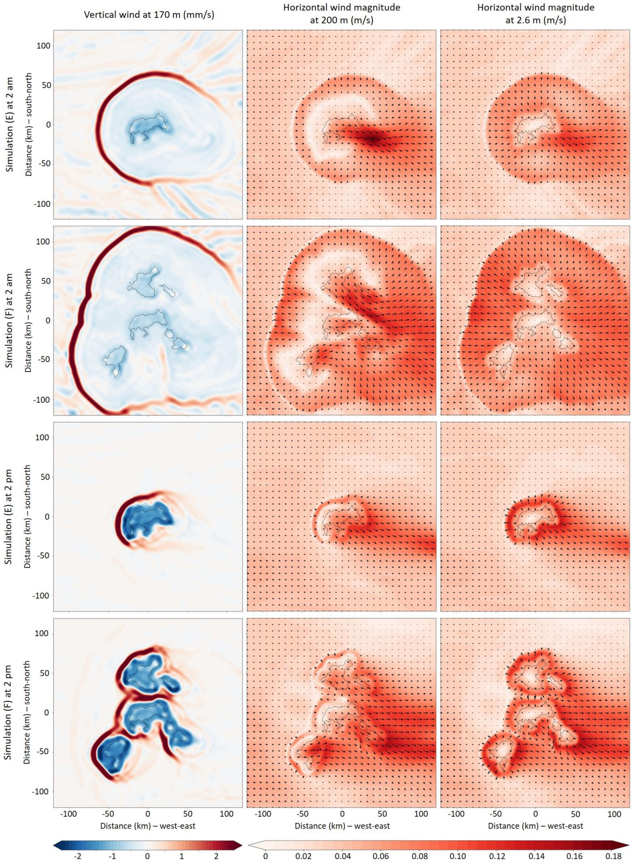
Figure 10. Maps, at 2 am and 2 pm, of vertical wind at 170 m and horizontal wind at 200 m and 2.6 m. Comparison of circulations obtained with a sole lake (simulation E) and the same lake (Oneida Lacus) surrounded by others (simulation F) with a background wind. The black dashed lines indicate the position of the lakes. The arrows indicate the direction and relative intensity of the horizontal wind.
