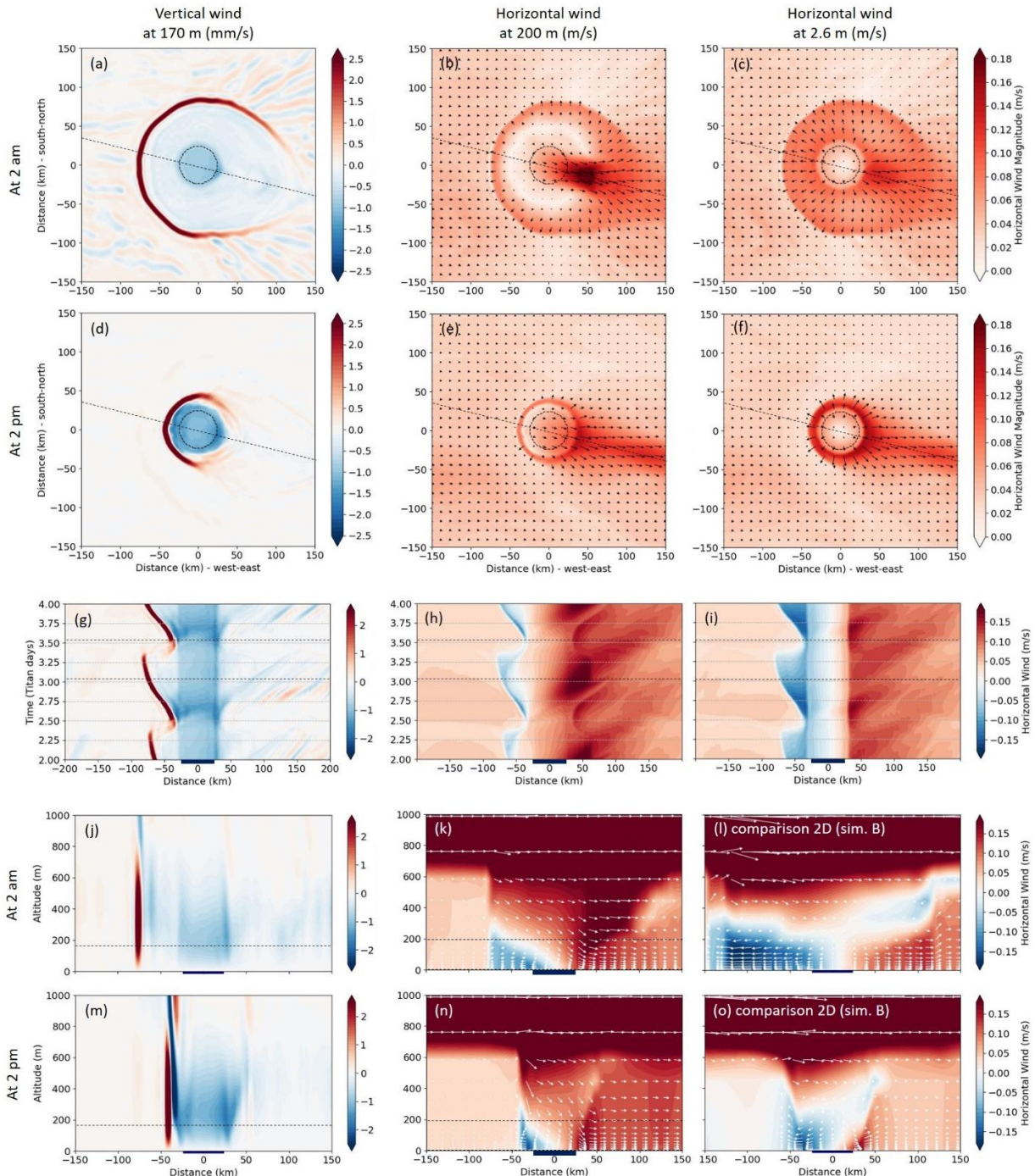
Figure 5. Horizontal and vertical winds. (a-k,m-n) Horizontal and vertical winds for simulation A, with a round lake of 50 km with GCM background winds. The black dashed circles (a-f) and blue line bars (g-o) indicate the position and size of the lake. The arrows indicate the direction and relative intensity of the wind. For (k,l,n,o) the vertical wind is x100 compared to the horizontal wind for sake of clarity. The dashed black lines on panels (a-f) indicate the position of the slices plotted with different axes on panels (g-o). Dashed black lines on panels (g-i) show the times in which panels (a-f) are plotted. Dashed black lines on panels (j, m) show the 170 m altitude level. Dashed black lines on panels (k) and (n) show the 2.8 and 200 m altitude levels. Panels (l) and (o) give wind results in the 2D case for comparison (simulation B).
