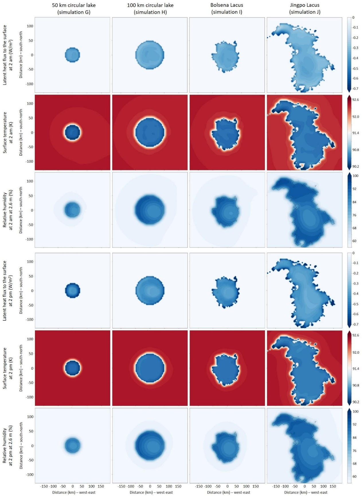
Figure 12. Maps, at 2 am and 2 pm, of latent heat flux to the surface, surface temperature and relative humidity at 2.6 m. Comparison of circulations obtained with a 50 km circular lake (simulation G), a 100 km circular lake (simulation H), Bolsena Lacus (simulation I) and Jingpo Lacus (simulation J) with a background wind. The black dashed line indicates the position of the lake.
