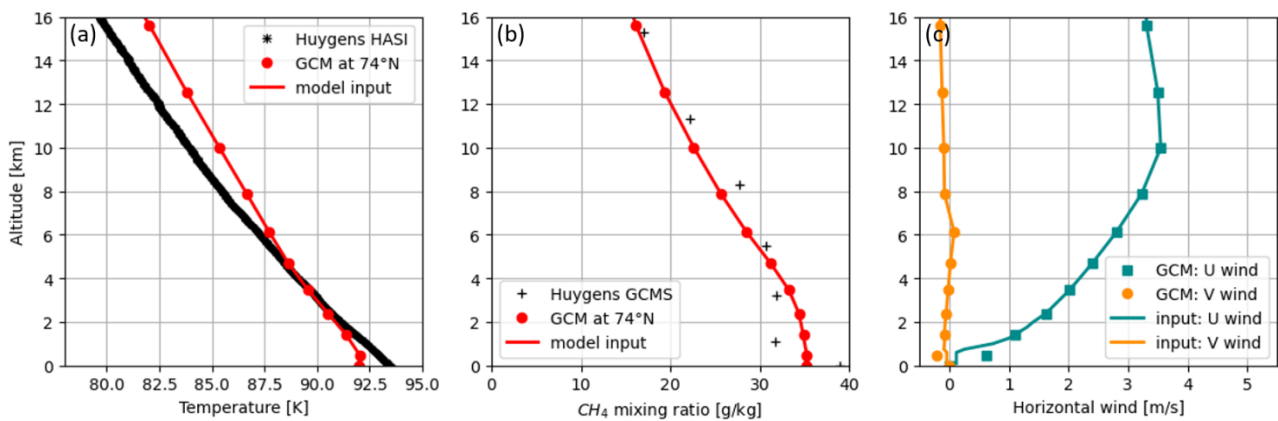
Figure 1. Temperature (a), methane mixing ratio (b), and horizontal wind (c) from Huygens HASI (Fulchignoni et al., 2005) and GCMS (Niemann et al., 2010) measurements at 10.6^\circ\text{S} just after the southern summer solstice, from the TAM GCM at 74^\circ\text{N} at the spring equinox (Lora et al., 2022), and used as inputs for our model.
