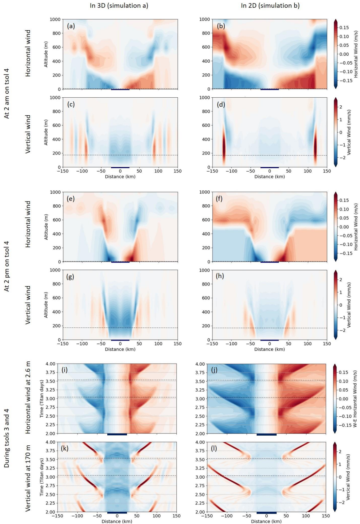
Figure 2. Horizontal and vertical winds as function of altitude, distance to the lake center and time. Comparison of circulations obtained in 3D (simulation a) and 2D (simulation b) for a 50 km diameter lake. Simulations start at midnight. The dark blue bars below the plots indicate the position and size of the lake. The black dashed lines indicate the position of the slices plotted with the different axes (with altitude from a to h, with time from i to l).
