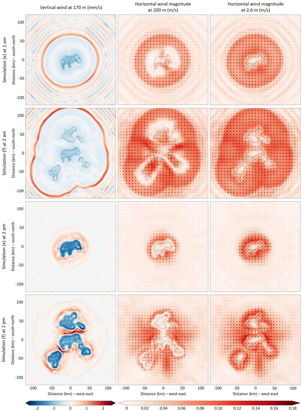
Figure 9. Maps, at 2 am and 2 pm, of vertical wind at 170 m and horizontal wind at 200 m and 2.6 m. Comparison of circulations obtained with a sole lake (simulation e) and the same lake (Oneida Lacus) surrounded by other lakes (simulation f) without background wind. The black dashed lines indicate the position of the lakes. The arrows indicate the direction and relative intensity of the horizontal wind.
