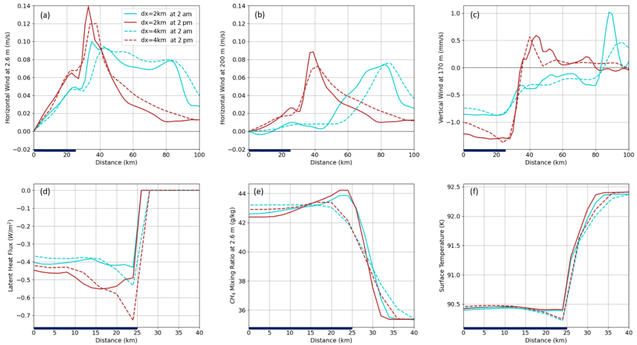
Figure A3. (a) Horizontal wind at 2.6 m, (b) at 200 m, (c) vertical wind at 170 m, (d) latent heat flux to the surface, (e) methane mixing ratio at 2.6 m, and (f) surface temperature, at 2 am (blue) and 2 pm (red). Solid lines are for the reference simulation done with a horizontal resolution dx of 2 km (simulation a). Dashed lines are for dx = 4 km (simulation g). Both simulations have a round lake of 50 km without background wind. The dark blue bars below the plots indicate the position of the lake.
