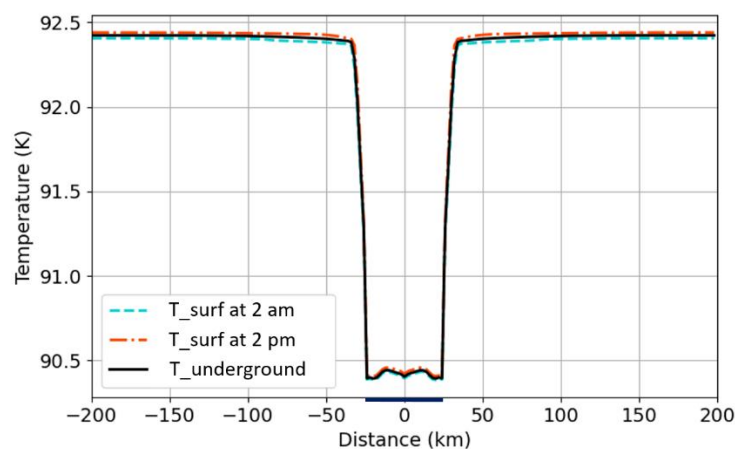
Figure A2. Surface temperature at 2 am and 2 pm, compared to the underground temperature in the case of a round lake of 50 km without background wind (simulation a). The dark blue bar below the plot indicates the position of the lake.
