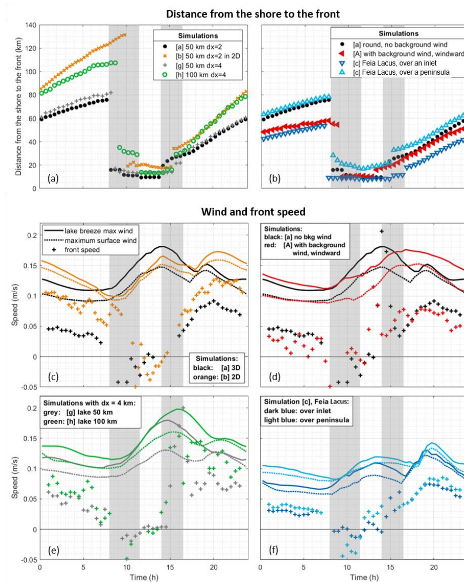
Figure 14. Comparison of the characteristics of the lake breeze in different simulations. (a,b) Distance from the shore to the front and (c,d,e,f) characteristic winds and front speed. Comparison of simulations a (reference: 50 km round lake without background wind, with a resolution dx = 2 km), A (with background wind), b (in 2D), c (Feia Lacus), g (resolution of dx = 4 km), and h (larger lake). Simulation details are given in Table 1 . Grey zones indicate times when the front is more diffuse.
