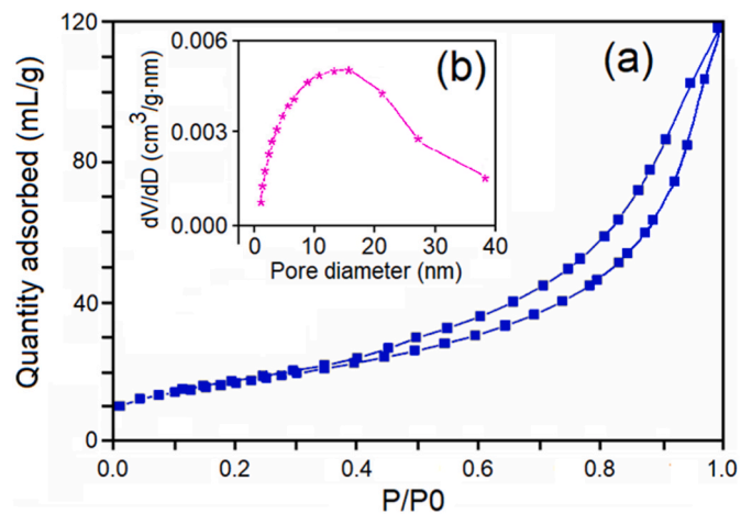
Fig. 5. The N 2 adsorption-desorption isotherms of the synthesized HAp-SB (a) and pore size distribution (b).
