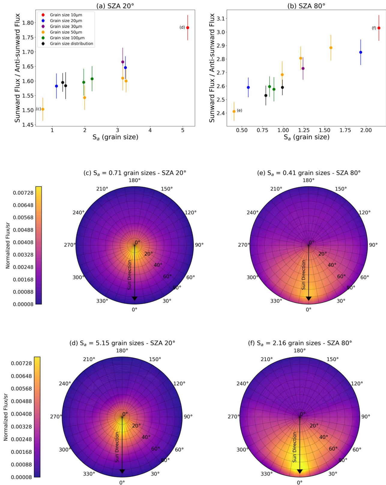
Figure 4. Sunward vs. anti-sunward fluxes ratio as a function of the average roughness evaluated for multiple regolith structures at SZA 20° (a) and 80° (b). Normalized angular distribution maps for two extreme regolith structures at SZA 20° (c) and (d), and at SZA 80° (e) and (f). The bottom half of each map represents the sunward direction hemisphere and the upper half the anti-sunward hemisphere. The error bars are based on the standard deviation of the ratios of protons launched from different random initial conditions.
