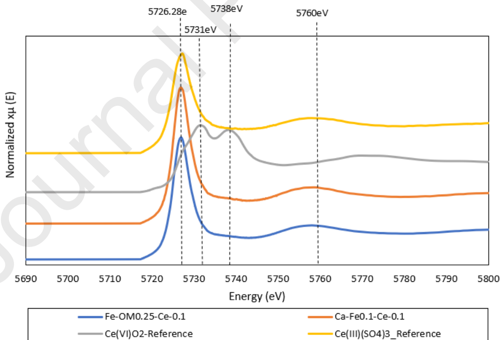
Figure 4. Ce L III -edge XANES spectra for samples and relevant references
