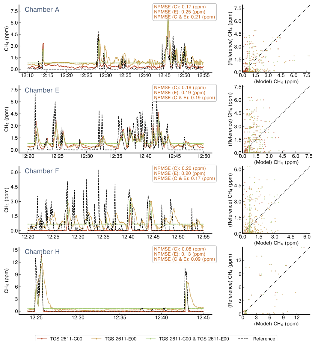
Figure A4. Reconstruction of release #2 using a MLP model. On left panels are shown the reconstructed CH 4 mole fractions for each chamber that captured the release, we present the reference signal (black dotted line), the reconstructed CH 4 mole fractions when the model has as input the TGS 2611-C00 sensor (red), the TGS 2611-E00 (yellow) or both types at the same time (green). The right panels show the 1:1 plot of the reference against the output of the model for the three configurations of inputs. Note the difference in the x-axis for the chambers.
