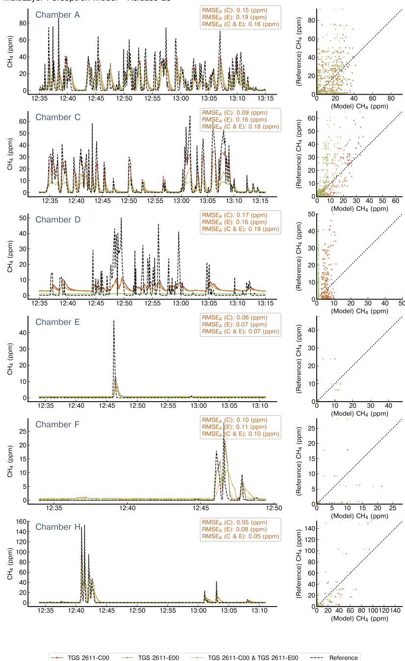
MultiLayer Perceptron Model - Release 25
