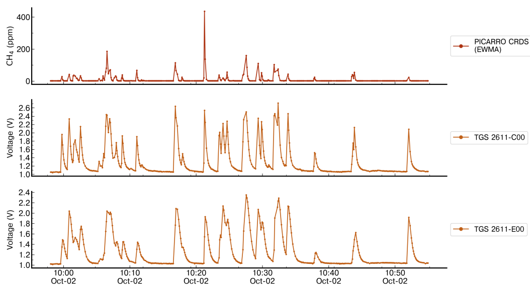
Figure A3. Comparison of the response of the TGS 2611-C00 and TGS 2611-E00 sensors with \text{CH}_4 measurements from the reference instrument for the release #2 which contains spikes with high concentration. The spikes observed on the TGS sensors corresponding from amplitudes between 100 ppm to more than 200 ppm are not distinguishable from spikes with amplitudes lower than 50 ppm.
