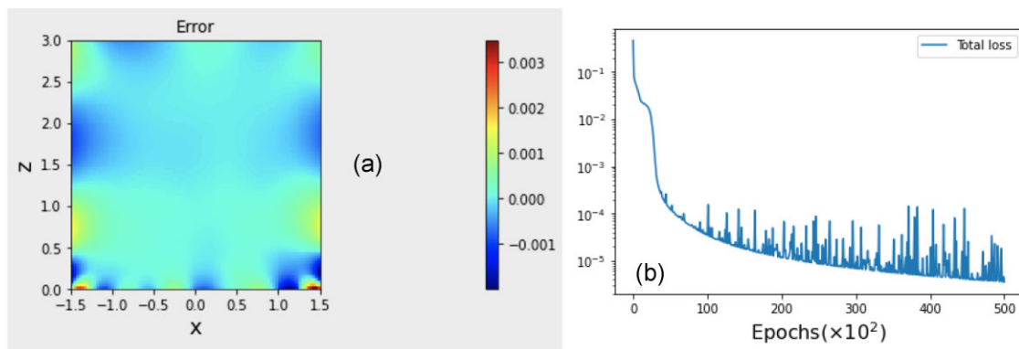
Figure 5. (a) Absolute error distribution (iso-contours of the difference between the PINNs and exact solutions) for the arcade case shown in the previous figure. (b) Corresponding evolution of the total loss function with the training epochs.
