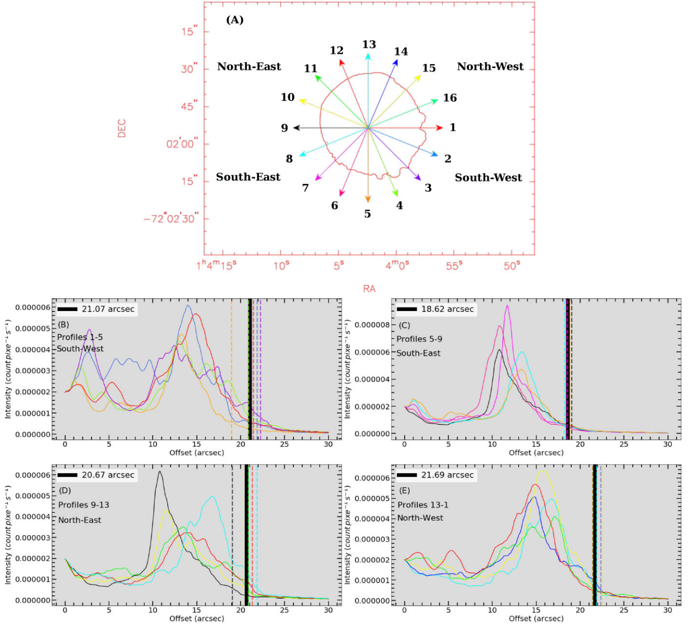
Figure 4. Estimate of X-ray radius of E0102. (A) Radial profiles overlaid on 3\sigma Chandra broadband X-ray image contour ( 6 \times 10^{-7} counts \text{pixel}^{-1} \text{s}^{-1} ). The central position of the remnant is RA (J2000) = 01^h 04^m 02.40^s , Dec (J2000) = -72^\circ 01' 53''.42 . (B–E) Radial profiles. The dashed vertical lines represent profile cut-offs and the thick black vertical lines represent the average of the cut-offs (in arcsec) for different parts of the shell; south-west, south-east, north-east, and north-west, respectively.
