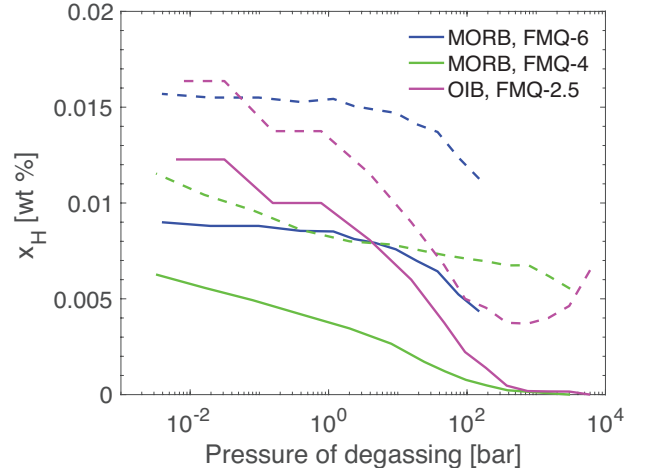
Figure 1. Degassing of H _2 from magma calculated by the magma degassing and speciation model of Gaillard & Scaillet (2014). We consider mid-ocean ridge basalt (MORB) with bulk H _2\text{O} content of 0.19 wt % and bulk CO _2 content of 0.16 wt %, degassing at the oxygen fugacities of FMQ-6 (corresponding to an undifferentiated planet) and FMQ-4 (corresponding to modern Mars), as well as ocean island basalt (OIB) with bulk H _2\text{O} content of 1 wt % and bulk CO _2 content of 0.3 wt %, degassing at the oxygen fugacities of FMQ-2.5. The solid lines count the degassing of H _2 and the dashed lines count the degassing of both H _2 and CO (with CO expressed in terms of its indirect effect on atmospheric H _2 , see text).
