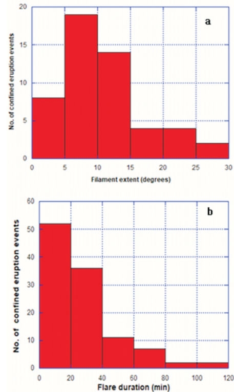
Fig. 2. a) Distribution of filament field extent for confined eruptions. b) Distribution of flare duration that results from confined eruptions
