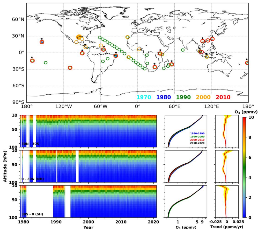
325 Figure 6. Top panel: Locations of the ozonesode stations in the tropics. The Southern Hemisphere Additional OZonesondes (SHADOZ) stations are marked with a black star (Bottom Left Panel): Ozone profiles from WOUDC ozonesonde averaged for the tropics, NH and SH, (Bottom Middle Panel) Mean distribution over each decade for each regions (Bottom Right Panel) and the yearly averaged trends for the period 1980–2020.
