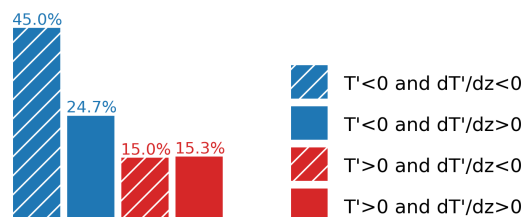
Figure 7. Fraction of cloudy BeCOOL lidar bins above 14.5 km within the four wave phases.
