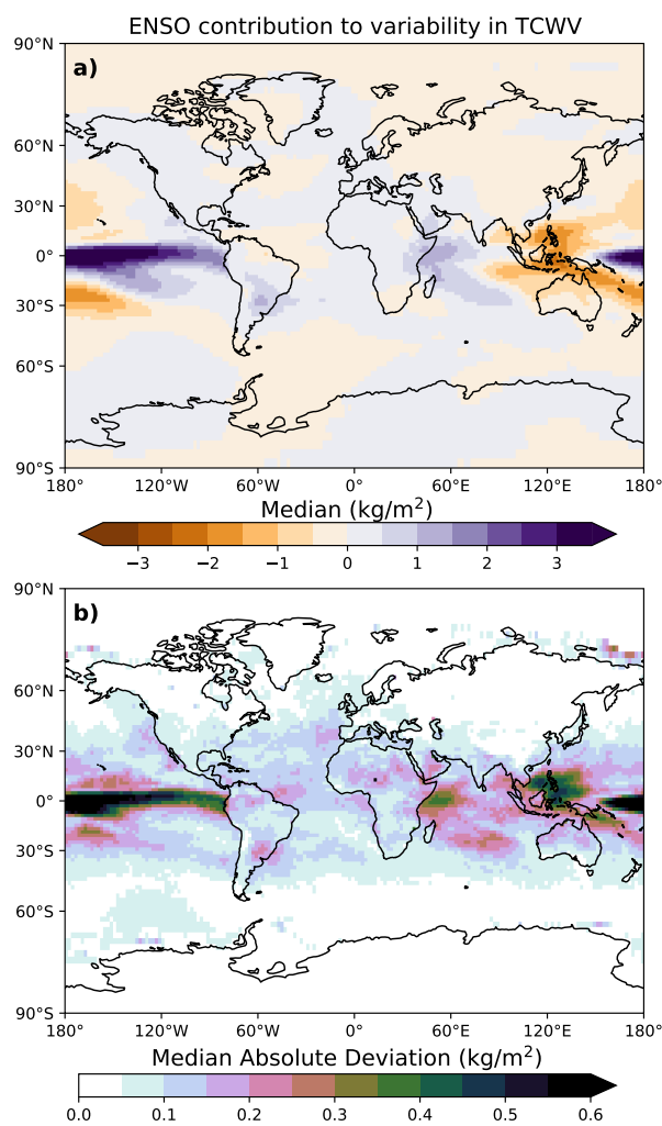
Figure 3. Archive ensemble median ENSO contribution to the variability in TCWV for the common long period (1988-2014) and median absolute deviation (MAD) to the ensemble median ENSO contribution.
