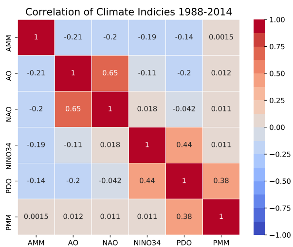
Figure 4. Correlation coefficients between the different climate indices used in this study for the period 1988 to 2014.
