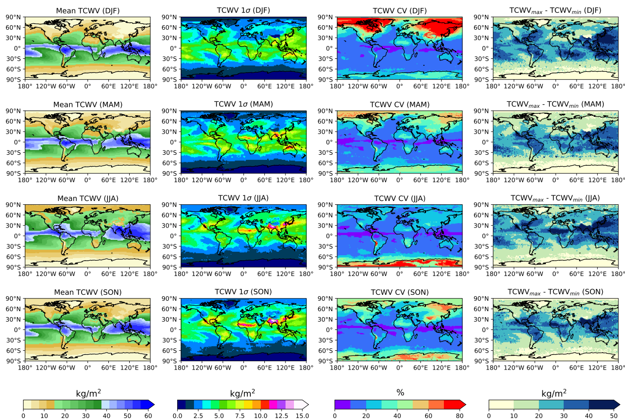
G-VAP Archive V2 Ensemble for the common period January 2005 to December 2009
