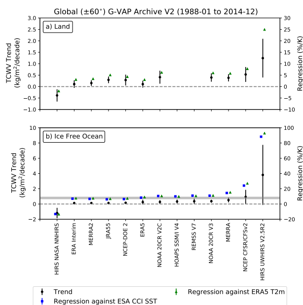
Figure 8. Trend estimates in total column water vapour (TCWV) in \text{kg/m}^2 per decade for data records that span the common 'long' period (1988-2014) for global land (a) and ice-free oceans (b) between \pm 60^\circ . Trends are represented as black dots with the estimated uncertainty of the trend shown in vertical bars. Also shown on the right-hand y-axes are the regression coefficient (%/K) for each data record. Regression has been carried out against sea surface temperature (SST) from the ESA Climate Change Initiative (CCI) and 2-metre air temperature (T2m) from ERA5. These are shown as blue squares and green triangles, respectively, with the regression error as vertical bars. The grey-shaded region on the bottom figure denotes the expected range of regression values and actual expectation based on the mean change in SST (Wentz and Schabel, 2000)
