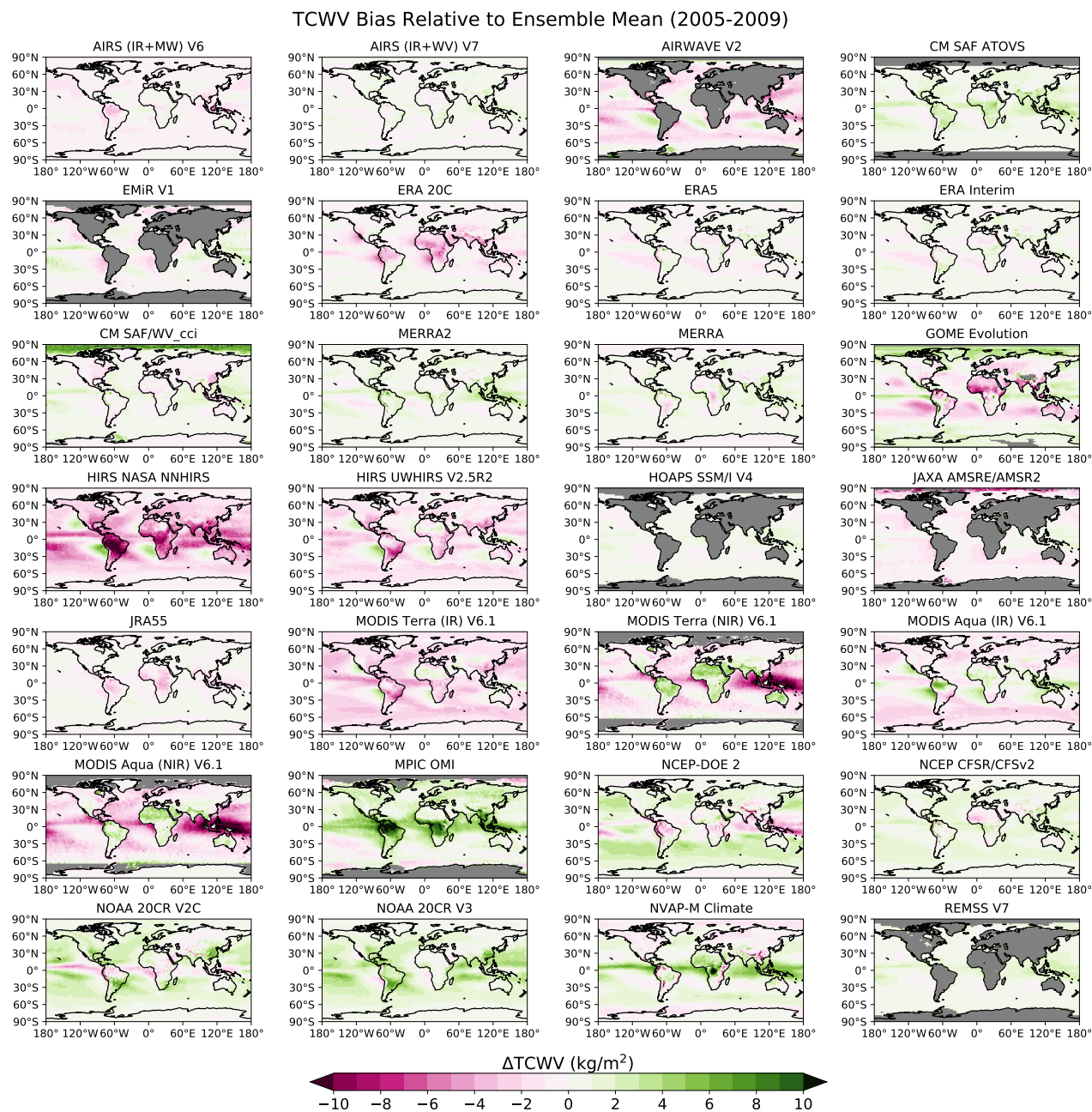
Figure 7. Ensemble member total column water vapour (TCWW) biases relative to the ensemble mean for the common period of all records (see Figure 1).
