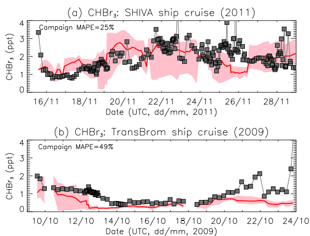
Figure 8. Comparison of modelled vs. observed \text{CHBr}_3 surface volume mixing ratio (ppt) during (a) SHIVA (2011) and (b) TransBrom (2009) ship cruises. The multi-model mean is shown and the shaded region is the model spread. The mean absolute percentage error (MAPE) over each campaign is annotated.
