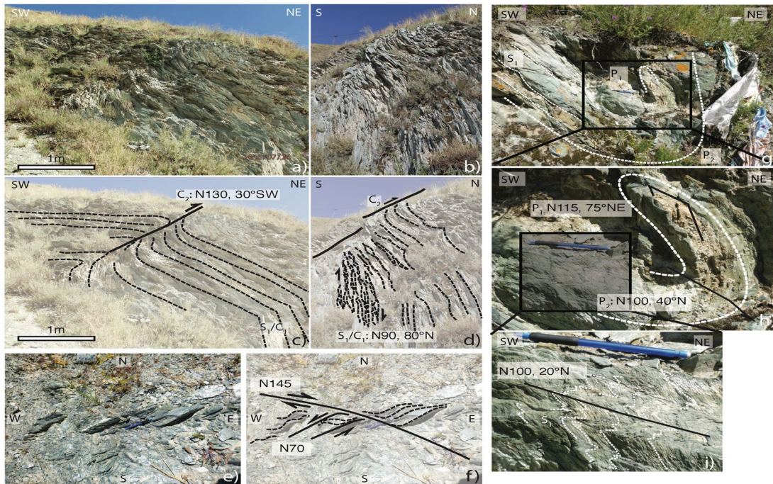
Figure 9. Ductile structures affecting blueschist-facies metabasalts on the Yushu monastery hill, north of the city (sampling sites of YU-15-16 and YU-15-17). (a, b) Field pictures and (c, d) structural interpretation: the main apparent subvertical foliation S_1 presents shear structures, suggesting that the foliation was transposed during a first deformation phase. This S_1/C_1 planes are affected by top-to-the-NE folding and shearing along C_2 planes. (e, f) View from above, the subvertical S_1 foliation is affected by conjugate strike-slip vertical shear zones, indicating N-S pure-shear flattening. (g–i) Interpreted field pictures of the two generations of folds. (h, i) Are close-up views of the fold structure showing the orientations of P_1 , P_2 and of the creulation axial planes.
