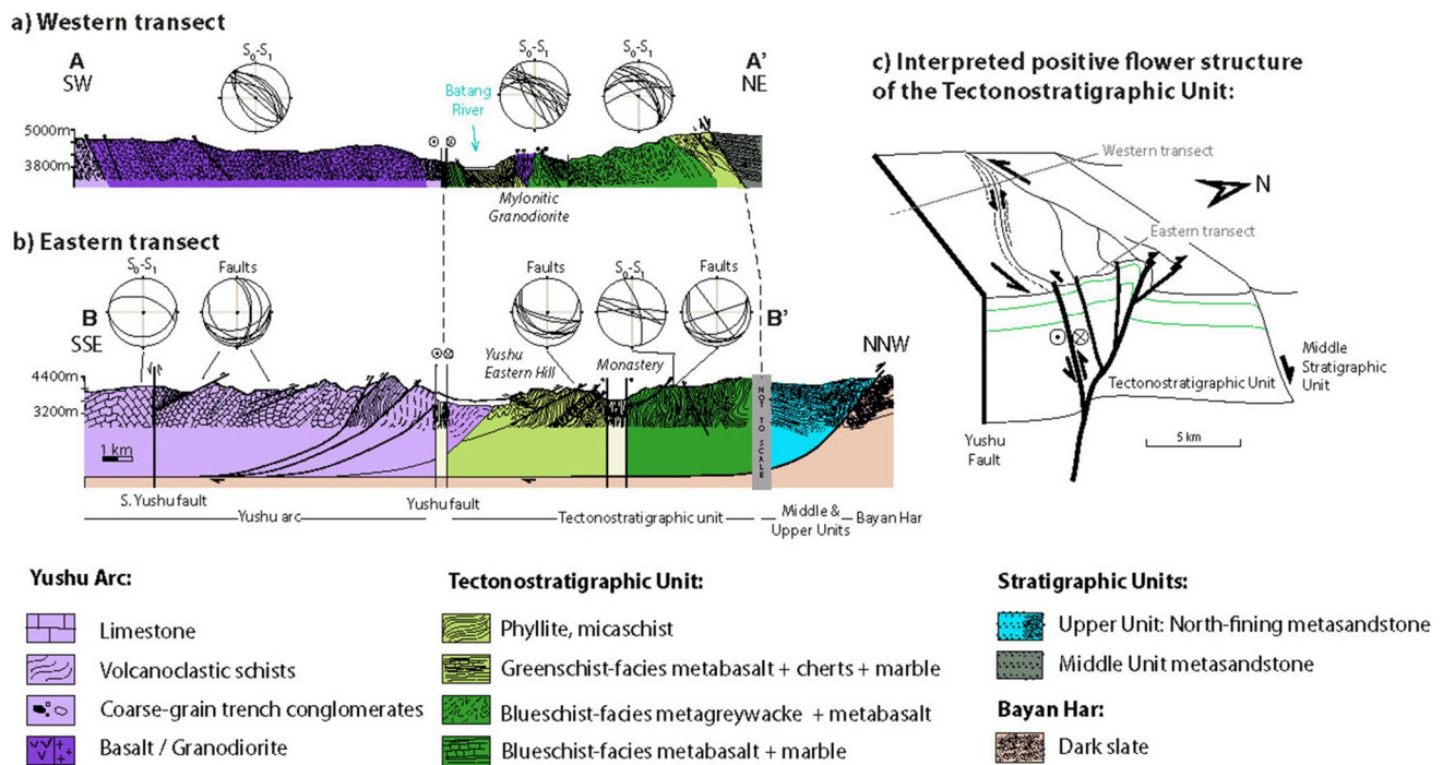
Figure 3. (a, b) Structural cross-sections of the Yushu mélange, with stereographic projections (lower hemisphere, equal area net) of the observed fabrics. (c) Schematic interpretation of the structures of the Tectonostratigraphic unit as part of a large-scale positive flower structure, resulting from regional transpressive deformation (see the text for explanation).
