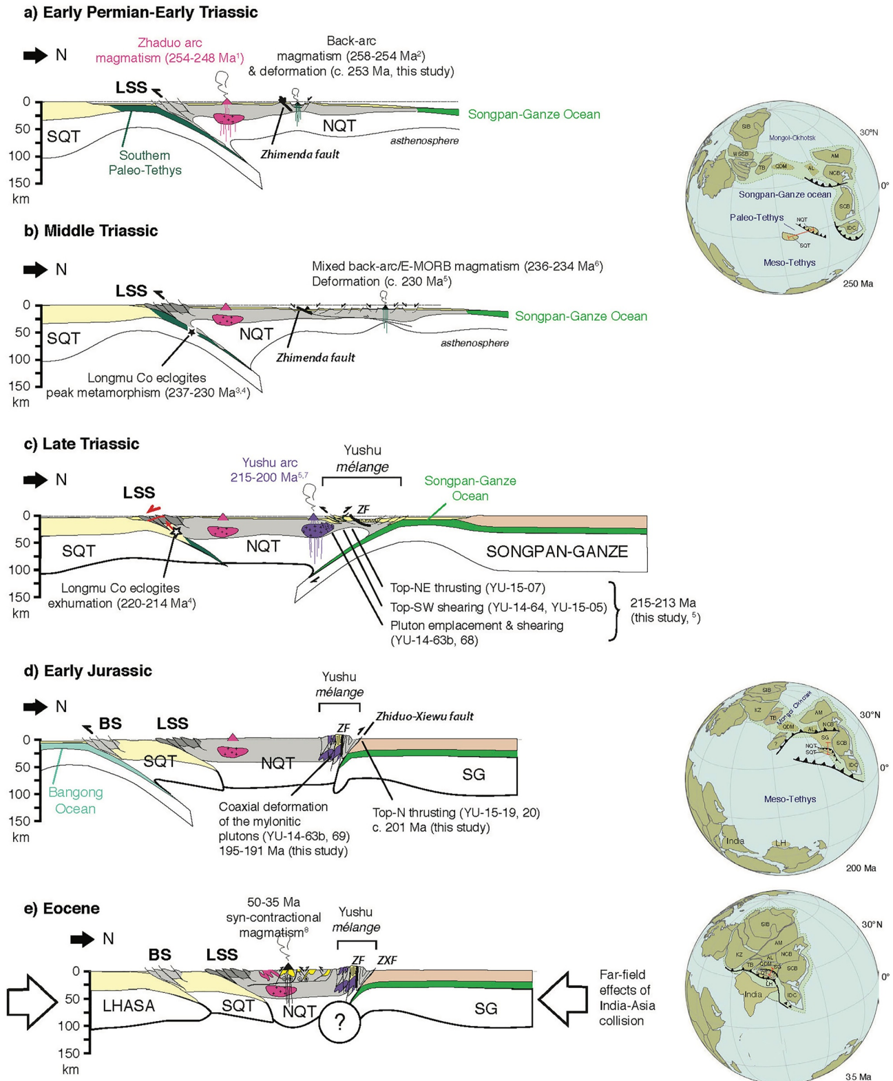
Figure 14. Schematic sketch (not to scale) of a possible geodynamic evolution of the Yushu area from the Permo-Triassic to the Eocene, reconciling the currently known ages of deformation and magmatism. Age data sources: (a) Yang et al. (2011); (b) H. Zhang et al. (2017); (c) Dan et al., 2018; (d) Q.-G. Zhai et al. (2011); (e) Yang et al. (2012); (f) B. Liu, Ma, Guo, Xiong, et al. (2016); (g) Roger et al. (2003); and (h) Spurlin et al., 2005. Abbreviations: CQMB, Central Qiangtang Metamorphic Belt; BS, blueschist facies; JS, Jinsha-Ganze-Litang Suture; LSS, Longmu Co-Shuangyu Suture; SQT, South Qiangtang; and NQT, North Qiangtang.
