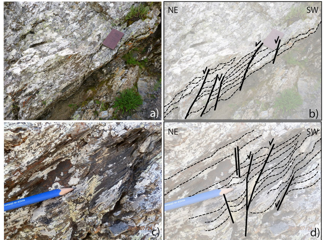
Figure 7. (a, c) Field pictures and (b, d) structural interpretations of top-to-the-NE normal shear within the hanging wall of the Zhimenda fault (sampling site of YU-15-11). Dashed lines indicate the main foliation planes, thick lines indicate shear planes.
