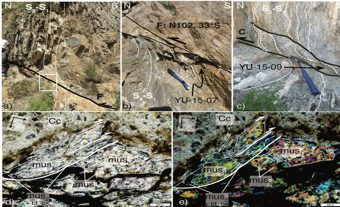
Figure 8. Top-to-the-north brittle structures affecting the subvertical S_0/S_1 schistosity on the eastern hill of the Yushu city. (a, b) Interpreted field picture of a fault plane on muscovite-bearing schists (sampling site of YU-15-07). (c) Interpreted field picture of a shear plane in cherts with quartz-chlorite and calcite veins (sampling site of YU-15-09). (d, e) Interpreted microphotographs of the fault plane sample YU-14-07, using (d) parallel light and (e) crossed Nicols. White dashed lines underline the foliation planes; solid white lines indicate glide planes or micro-thrusts between grains; white dotted lines delineate muscovite grain boundaries. mus_1 are deformed porphyroclasts, mus_2 and mus_3 are syn-deformation (re)crystallized grains. Mineral abbreviations: Cc, carbonate; bt, biotite; ox, oxide; mus, muscovite; and qz, quartz.
