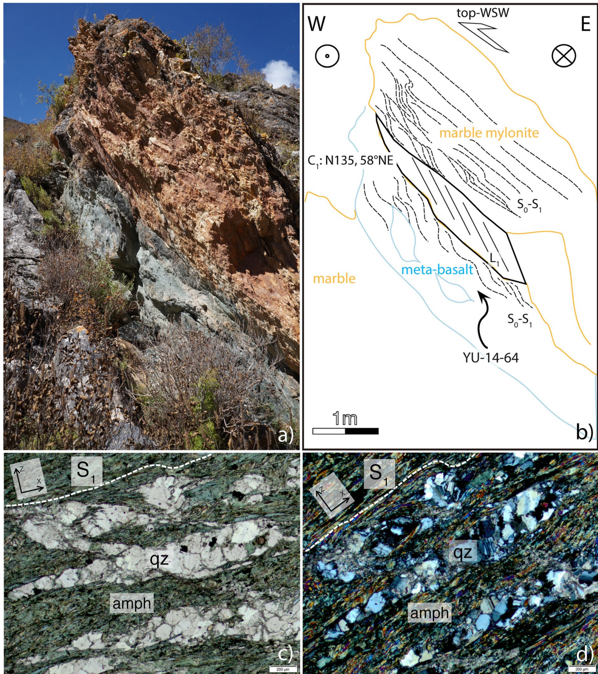
Figure 6. (a) Field picture and (b) structural interpretation of a top-to-the-WSW transpressive shear contact between marble and blueschists with metabasalt lenses (sampling site of YU-14-64). (c, d) Interpreted microphotographs of the metabasaltic sample YU-14-64 using (c) parallel light and (d) crossed Nicols. The main foliation plane S_1 is underlined with a white dashed line. Mineral abbreviations: amph, amphibole; qz, quartz; and plg, plagioclase.
