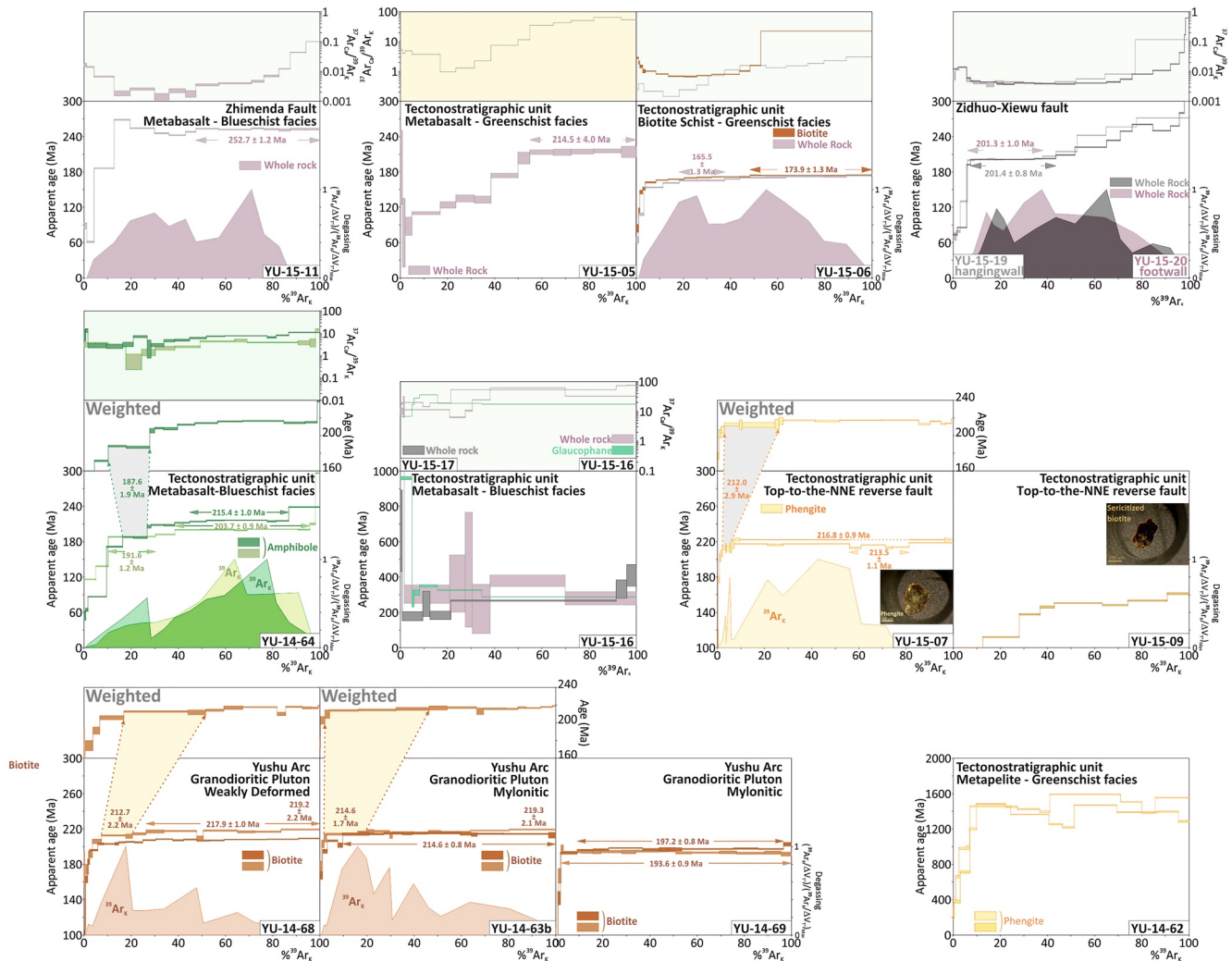
Figure 12. ^{40}\text{Ar}/^{39}\text{Ar} apparent age spectra of minerals and/or whole-rock fractions from deformed rocks from the Yushu mélangé. Apparent age error bars are at the 1 \sigma level; Errors in the J-parameter are not included. Plateau and pseudo-plateau ages ( 2\sigma uncertainties including errors in the J-parameter) are given when applicable. ^{39}\text{Ar}_K degassing spectra ( (^{39}\text{Ar}_K/\text{DVT})/(^{39}\text{Ar}_K/\text{DVT})_{\text{Max}} versus \%^{39}\text{Ar}_K ) are provided for most of the experiments (See Tremblay et al. (2020) for a detailed explanation).
