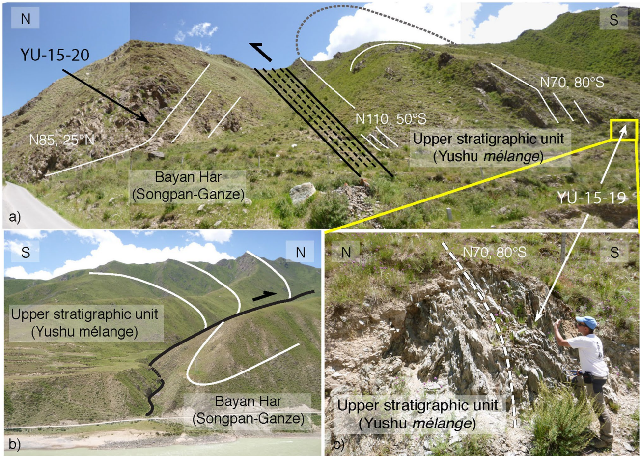
Figure 10. Top-to-the-north contact between the Yushu mélangé upper stratigraphic unit and the Bayan Har turbidites of the Songpan-Ganze block, in the Zhiduo-Xiewu fault zone: (a, c) outcrop views, with measured structural data reported (sampling site of YU-15-19 and YU-15-20); (b) landscape view.
