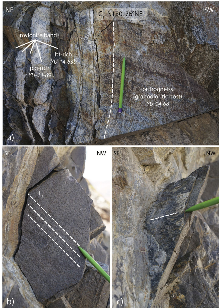
Figure 4. Outcrop pictures of the mylonitic granodiorite pluton (western transect). (a) Heterogeneous composition of the pluton, with mylonite bands wrapping a much less deformed granodiorite lens. The main C_1 shear planes direction is indicated. (b) Surface of a C_1 plane within a mylonitic band, showing L_1 lineation defined by the alignment of tiny biotite flakes. (c) Late sub-horizontal brittle striation on a slickenside, corresponding to a C_1 plane, and related to the present-day activity of the Yushu fault.
