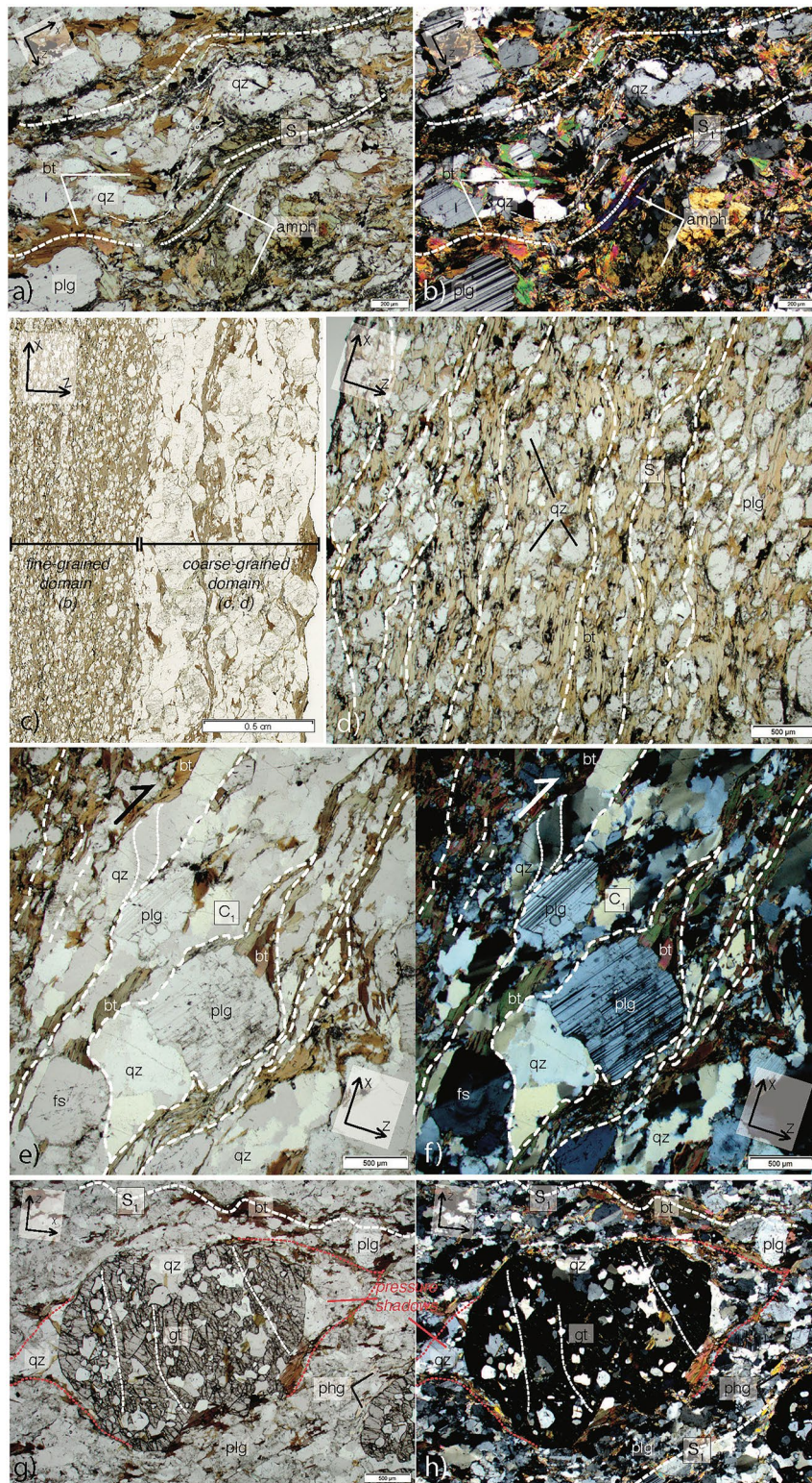
Figure 5. Interpreted optical microphotographs of samples from the mylonitic granodiorite pluton. S_1 foliation is underlined by white dashed lines; stretching direction (X) is N130. (a, b) Least deformed part of the granodiorite pluton (sample YU-14-68), using parallel light and crossed Nicols. (c) Thin-section scan showing the contact between a fine-grained mylonitic band (left) and a coarse-grained orthogneiss domain (right). (d) Fine-grained mylonitic band (sample YU-14-63b), using parallel light. (e, f) Coarse-grained domain, using parallel light and crossed Nicols; the internal deformation of quartz grains is underlined. (g, h) Garnet-bearing, quartz-rich mylonite band (sample YU-14-69), using parallel light and crossed Nicols; red dotted lines delineate pressure shadows. Mineral abbreviations: amph, amphibole; bt, biotite; fs, alkali feldspar; gt, garnet; plg, plagioclase; and qz, quartz.
