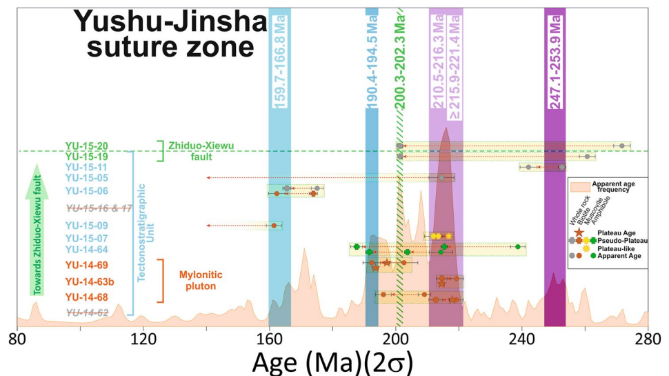
Figure 13. Synthesis of plateau, pseudo-plateau, plateau-like, and apparent ages ( 2\sigma error bars) from ^{40}\text{Ar}/^{39}\text{Ar} analyses of whole rock (gray), biotite (brown), phengite (yellow), and amphibole (green) single grains from samples from the Tectonographic Unit and the Zhiduo-Xiewu fault plotted against the frequency histogram (probability density diagrams) of the apparent ages (see Tremblay et al. (2020) for explanation). The samples are classified according to their sampling distance from the Zhiduo-Xiewu Fault. The main events identified by the ^{40}\text{Ar}/^{39}\text{Ar} geochronological study are highlighted by color bars following the color codes of the International Chronostratigraphic Chart. The significance of these periods is discussed in the text.
