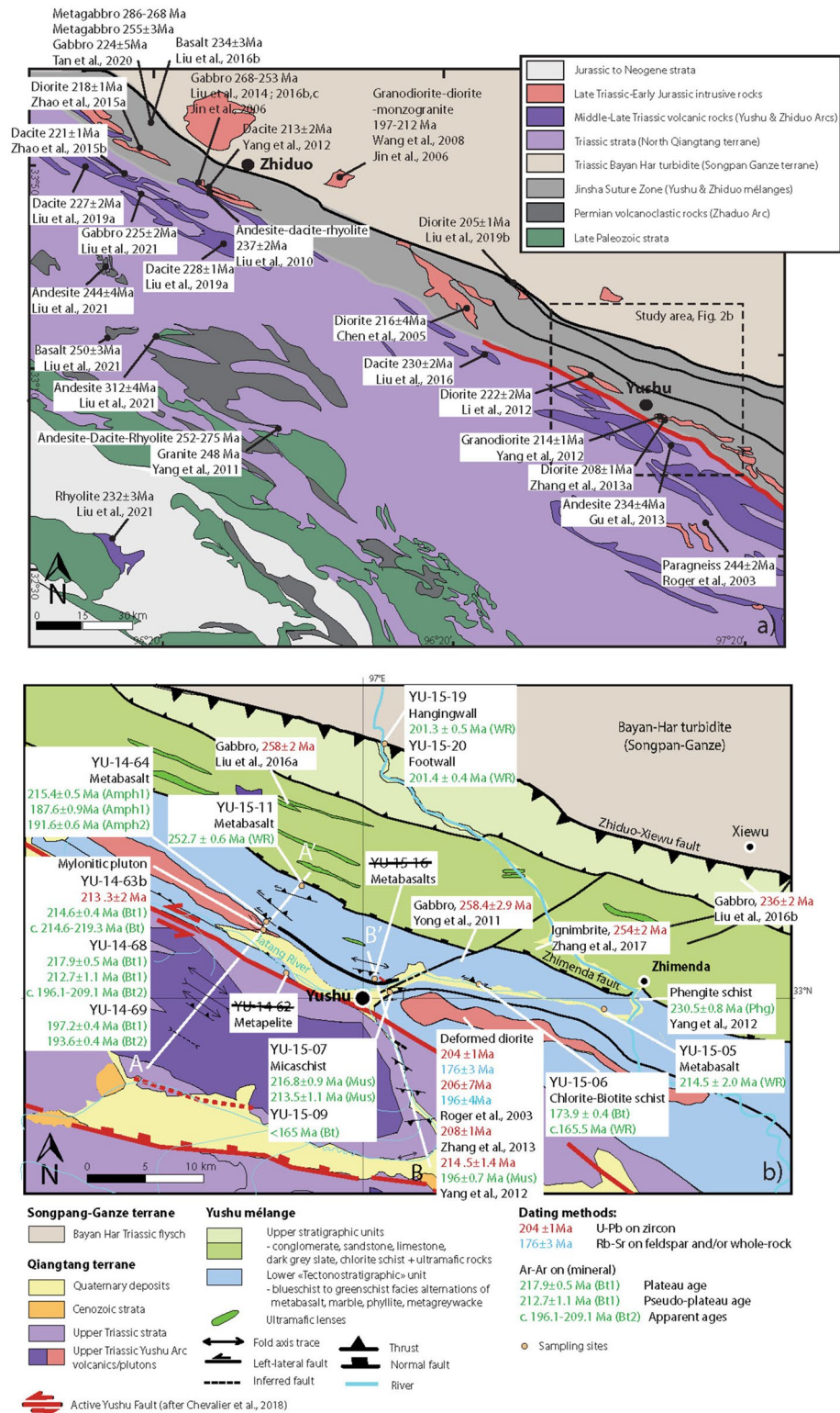
Figure 2. (a) Geological map of the Yushu-Zhiduo area in northeastern Qiangtang, showing the distribution of recently dated Mesozoic magmatic rocks along the Western Jinsha Suture. Modified from Y. Liu et al. (2021) and Yang et al. (2014). The location of our study area is indicated by the insert. (b) Map of the Yushu mélangé and adjacent areas, modified from Yang et al. (2012), H. Zhang et al. (2017), and the Geological Survey of Qinghai Province 1:250000 Geological Map (2005), according to our observations. Available age data for magmatic and deformed rocks are reported. AA' and BB' indicate respectively the western and eastern cross-sections of Figures 3a and 3b.
