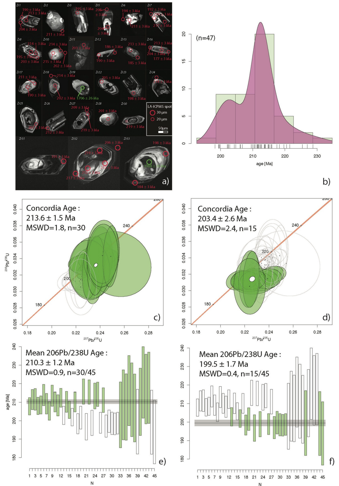
Figure 11. Zircon LA-ICP-MS U-Pb isotopic data and results for the mylonitic granodiorite sample YU-14-63b. (a) Zircons morphologies in CL microscopy, with laser-ablation spot locations. (b) Zircon U-Pb age probability plots. (c, d) Tera-Wasserburg concordia diagrams and (e, f) mean ^{206}\text{Pb}/^{238}\text{U} age plots; the left panels (c, e) corresponds to the 30 oldest analyses, the right panels (d, f) to the 15 youngest.
