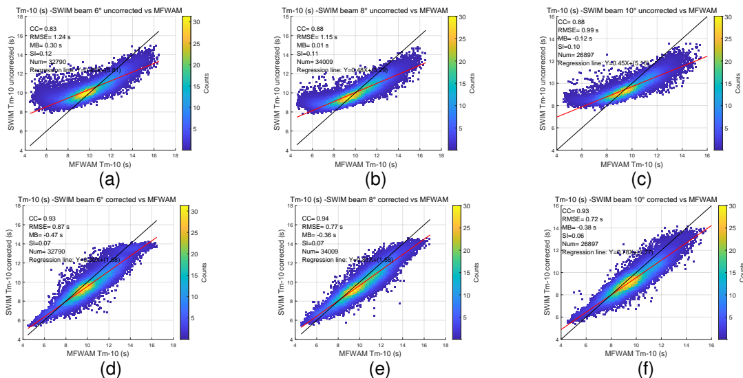
Fig. 9. Same as Fig. 7, but for cases of pure swell.
