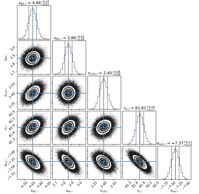
Fig. A.2. Posterior distribution of the parameters describing the total intensity of the disc with NICMOS.
