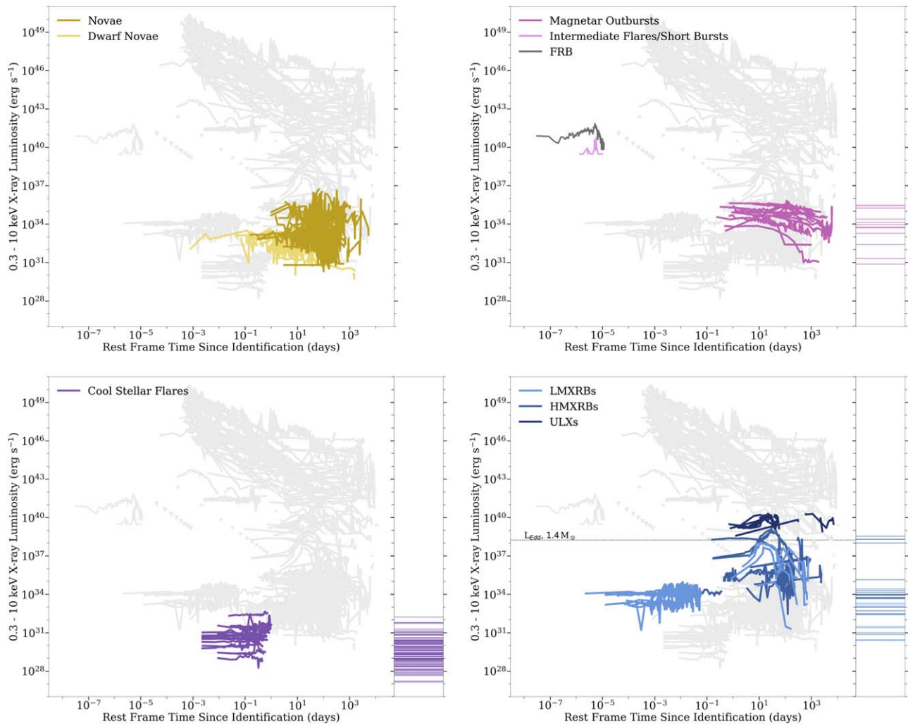
Figure 4. X-ray phase space of Galactic (CVs, magnetar flares/outbursts, and cool stellar flares) and Galactic/extragalactic (XRBs, ULXs, and FRBs) transients and variables, including those classes of event with some signals that have been observed to originate within the Galaxy, such as CVs (novae and dwarf novae), magnetar flares and outbursts, FRBs (specifically the Galactic FRB 200428), cool stellar flares, XRBs, and ULXs. We underplot the Eddington luminosity for a 1.4 M_{\odot} progenitor for additional context in the XRBs/ULX panel. With the exception of the CV panel, at right, we show quiescent luminosities for each class of object. Included events are listed in Tables A6–A9.
