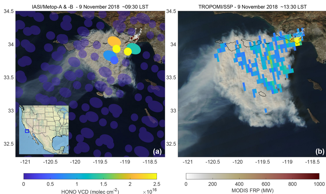
Figure 14. HONO VCDs (in molec cm -2 ) from IASI/MetOp-A and -B (~9:30 LST overpass) and TROPOMI (~13:30 LST overpass) during the Woolsey Fire, California, on 9 November 2018. The shape of each IASI dot corresponds to the on-ground footprint of an individual measurement. The dark-blue, semi-transparent IASI pixels indicate measurements without HONO detections and allow us to visualize the difference in spatial sampling between IASI and TROPOMI. The small white-to-red dots indicate the FRP values of active fires detected by MODIS/Terra (~10:30 LST) and MODIS/Aqua (~13:30 LST), coincident with the IASI and TROPOMI measurements, respectively. Visible imagery from MODIS/Terra (a) and MODIS/Aqua (b).
