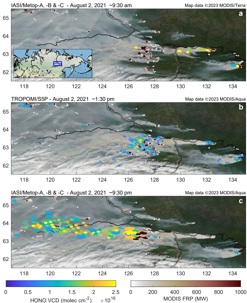
Figure 15. HONO VCDs (in \text{molec cm}^{-2} ) from IASI/Metop-A, -B and -C (~9:30 am and pm overpasses, separately) and TROPOMI (~1:30 pm overpass) during Siberian wildfires on August 2, 2021. The shape of each IASI dot corresponds to the footprint on ground of an individual measurement. The small white/reddish dots indicate the FRP values of active fires detected by MODIS/Terra (~10:30 am and pm, separately) and -Aqua (~1:30 pm), coincident with the IASI and TROPOMI measurements, respectively. Base maps are from MODIS/Terra and -Aqua visible imagery.
