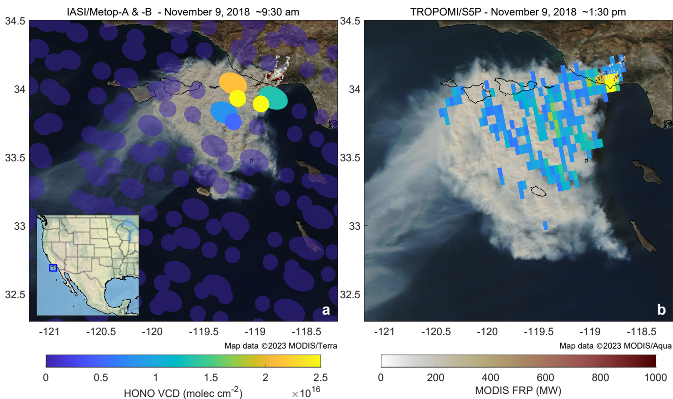
Figure 14. HONO VCDs (in molec \text{cm}^{-2} ) from IASI/Metop-A and -B ( \sim 9:30 am overpass) and TROPOMI ( \sim 1:30 pm overpass) during the Woolsey Fire, California, on November 9, 2018. The shape of each IASI dot corresponds to the footprint on ground of an individual measurement. The dark blue, semi-transparent IASI pixels indicate measurements without HONO detections and allow to visualize the difference of spatial sampling between IASI and TROPOMI. The small white/reddish dots indicate the FRP values of active fires detected by MODIS/Terra ( \sim 10:30 am) and -Aqua ( \sim 1:30 pm), coincident with the IASI and TROPOMI measurements, respectively. Base maps are from MODIS/Terra and -Aqua visible imagery.
