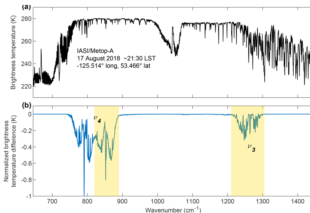
Figure A1. Typical IASI spectrum (displayed in brightness temperature) in the 645\text{--}1445 \text{ cm}^{-1} spectral range (a) and the Jacobian of the \nu_4 and \nu_3 HONO spectral absorption bands in the thermal infrared (b). The 820\text{--}890 and 1210\text{--}1305 \text{ cm}^{-1} spectral ranges used for the calculation of the two HONO HRIs are illustrated in coloured rectangles. The brightness temperatures were normalized to have a minimum value of -1 for visibility purposes. The Jacobian has been produced by the line-by-line radiative transfer model Atmosphit for a standard atmosphere.
