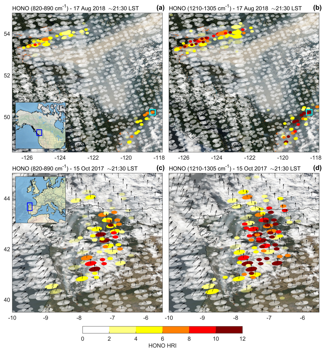
Figure 1. HONO HRIs from single IASI/MetOp-A and -B nighttime overpasses ( \sim 21:30 LST) over wildfires in British Columbia, Canada, on 17 August 2018 (a–b) and in Spain/Portugal on 15 October 2017 (c–d). The HRIs have been calculated in the 820\text{--}890 and 1210\text{--}1305\text{ cm}^{-1} spectral ranges. The shape of each dot corresponds to the on-ground footprint of an individual IASI measurement. The observations with \text{HRI} < 4 are displayed with semi-transparency. The vectors in the bottom panels represent the ECMWF ERA5 daily horizontal wind fields at the planetary boundary layer height. The small orange dots indicate the active fires detected by MODIS/Terra ( \sim 22:30 LST). The base map is from MODIS/Aqua visible imagery ( \sim 13:30 LST). The light-blue square in panels (a) and (b) points to the IASI/MetOp-A spectrum analysed in Sect. 4.2, with visible imagery from MODIS/Aqua.
