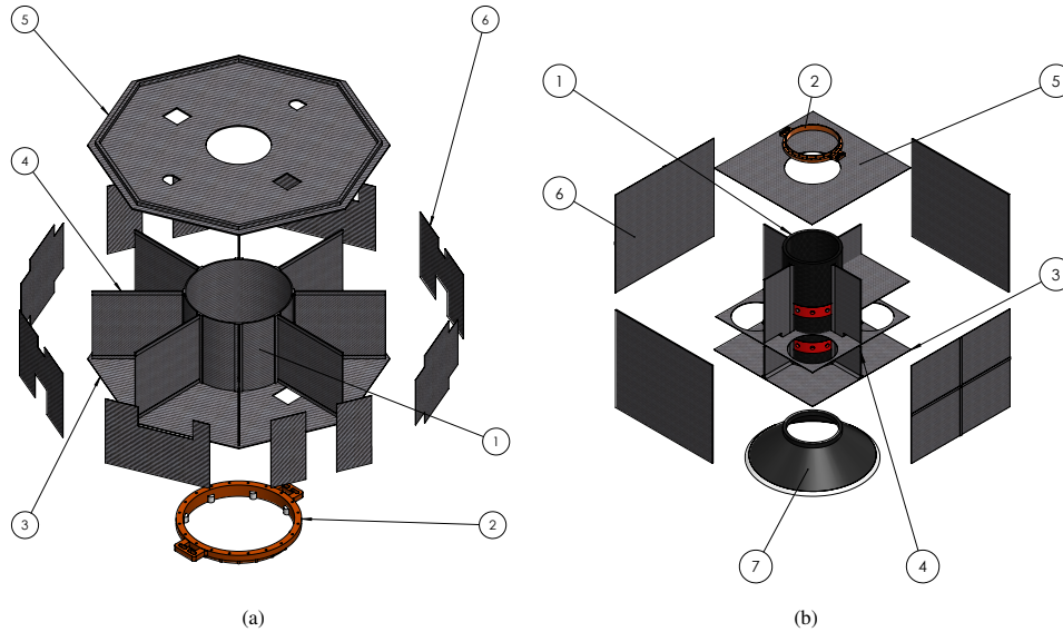
Figure 5: Structure of both spacecraft types (not to scale). (a) Scientific spacecraft structure. (b) Transfer vehicle structure. Legend: (1) Central Core, (2) Satellite Separation Ring, (3) Bottom Panel, (4) Shear Panel, (5) Top Panel, (6) Side Panel and (7) Payload Adapter.
