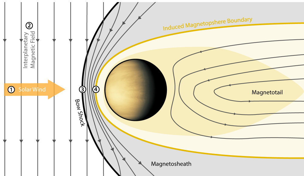
Figure 1: Conceptual overview over the Venusian induced magnetosphere. The numbers indicate the different plasma regions: 1. the solar wind, 2. IMF, 3. Bow shock, 4. IMB
