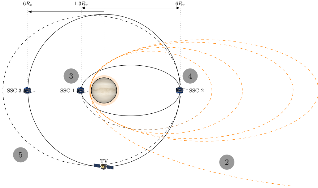
Figure 3: Mission phases at Venus as described in Section 4.
