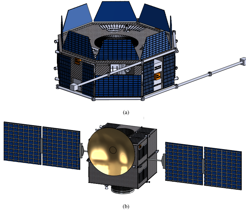
Figure 4: Spacecrafts in the deployed configuration (not to scale). (a) Scientific spacecraft. (b) Transfer vehicle structure.
