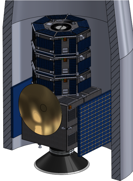
Figure 2: Scheme of the stacked configuration inside the Ariane's fairing.
