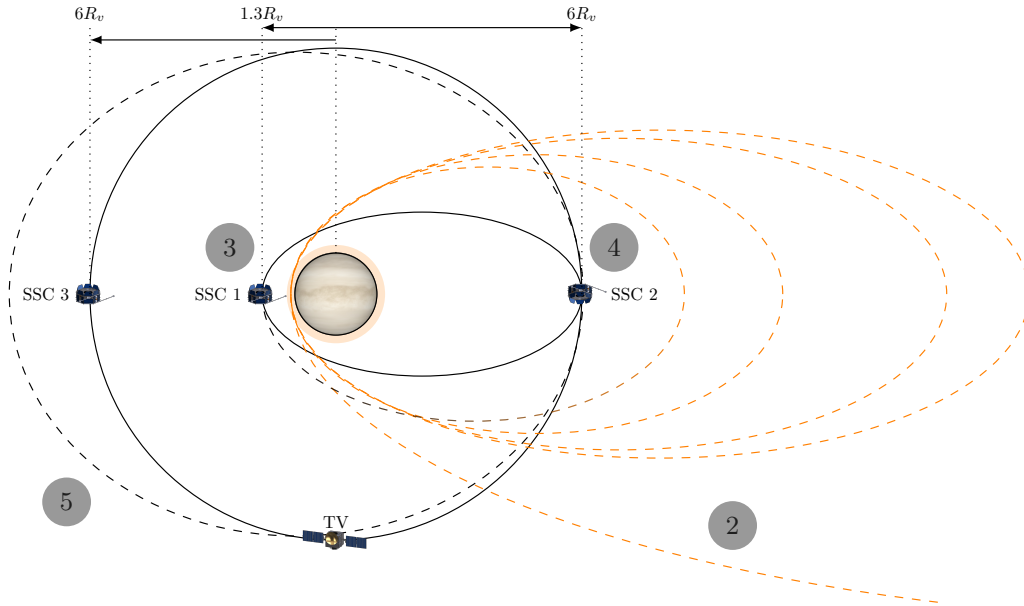
Figure 3: Mission phases at Venus as described in Section 4.
