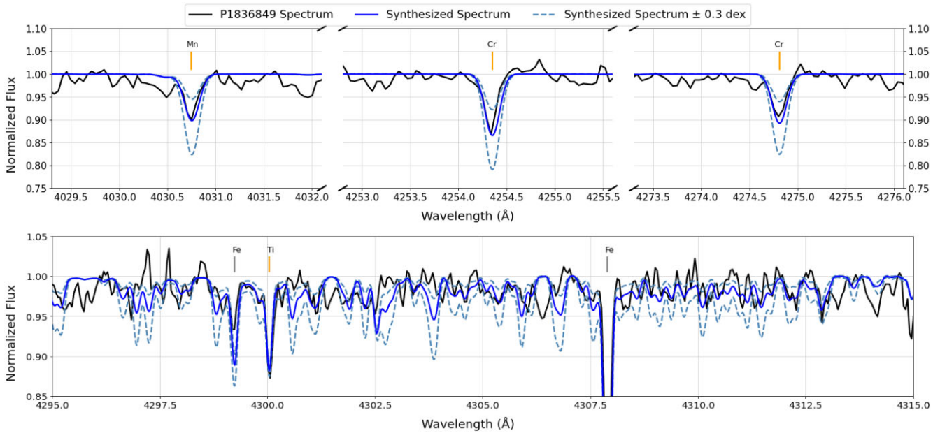
Figure 3. Upper Panels: The Mn I and two Cr I lines used in this analysis are shown, including our best-fitting syntheses, and \Delta[X/Fe] \pm 0.3 . Though the lines are weak ( \lesssim 30 mÅ each), they are clear and well modelled. Lower Panel: The G band including our best upper-limit syntheses, with ^{12}\text{C}/^{13}\text{C} = 40 (EMP dwarf; e.g. Spite, Spite & Barbuy 2021) and [\text{C}/\text{Fe}] = +0.8 . Two more syntheses show \Delta[\text{C}/\text{Fe}] \pm 0.3 . One Ti II line used in this analysis (orange) and two Fe I lines not used (grey) are also indicated. The plot is zoomed in for clarity.
