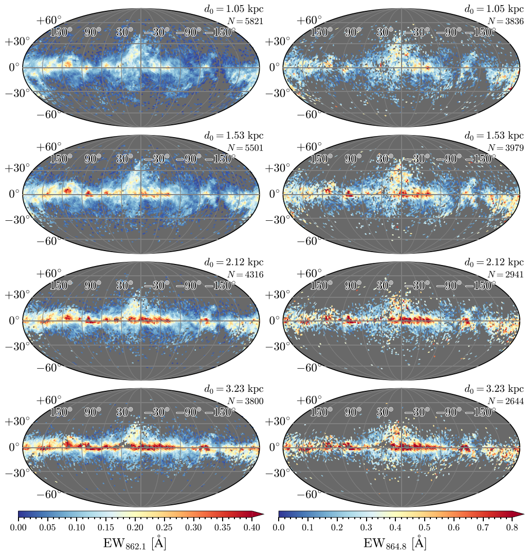
Fig. 20. Galactic distributions of EW_{862.1} ( left panels ) and EW_{864.8} ( right panels ) from DIB results in FPR in Mollweide projection at HEALPix level 5, at four distances. The distance ( d_c ) and the number of voxels ( N ) are indicated in each subpanel.
