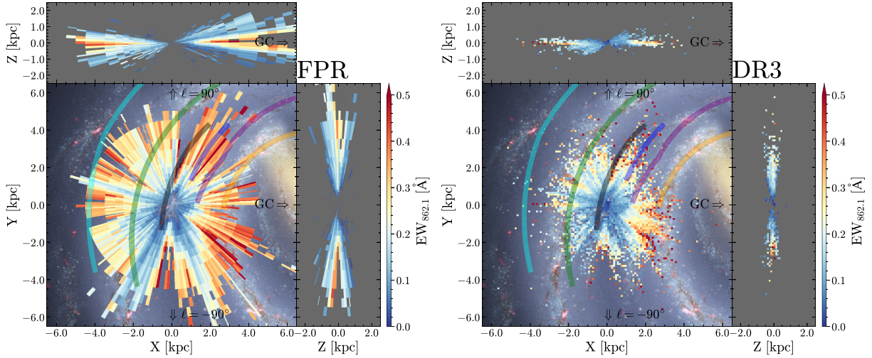
Fig. 19. Distribution of EW_{862.1} in the Galactic plane (XY), meridian plane (XZ), and rotational plane (YZ) for the FPR results ( left panel ) and the DR3 results ( right panel ), respectively, plotted over the Milky Way sketch created by Robert Hurt and Robert Benjamin (Churchwell et al. 2009). Some log-periodic spiral arms described in Reid et al. (2019) are also presented by coloured lines: Scutum–Centaurus Arm in orange; Sagittarius–Carina Arm in purple; Local Arm in black; Perseus Arm in green; Outer Arm in cyan; and the spur between the Local and Sagittarius–Carina arms in blue. The Galactic centre is located at (X, Y, Z) = (8.15, 0, 0) .
