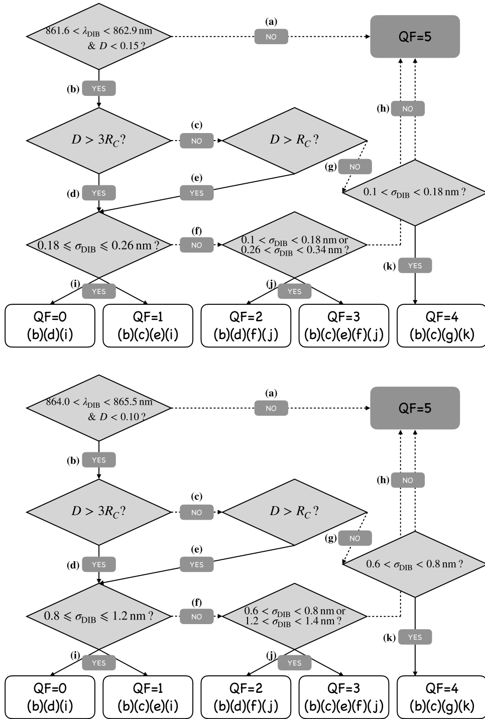
Fig. 9. Flowchart of the criteria to generate quality flags (QFs) for DIBs \lambda_{862.1} (upper panel) and \lambda_{864.8} (lower panel), respectively. The flag numbers and the corresponding arrow paths for classification are listed in the bottom box in each panel.
