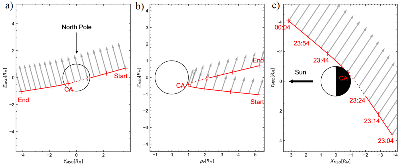
Figure 2. BepiColombo first Mercury flyby as seen (a) from the Sun, (b) in a Z-\rho Z plane in the MSO reference frame and (c) looking down on Mercury's orbit plane. The black circle represents the planet, the gray arrows the boresight of PHEBUS FoV and the red line the spacecraft trajectory. The red dotted line represents the transit in Mercury's shadow.
