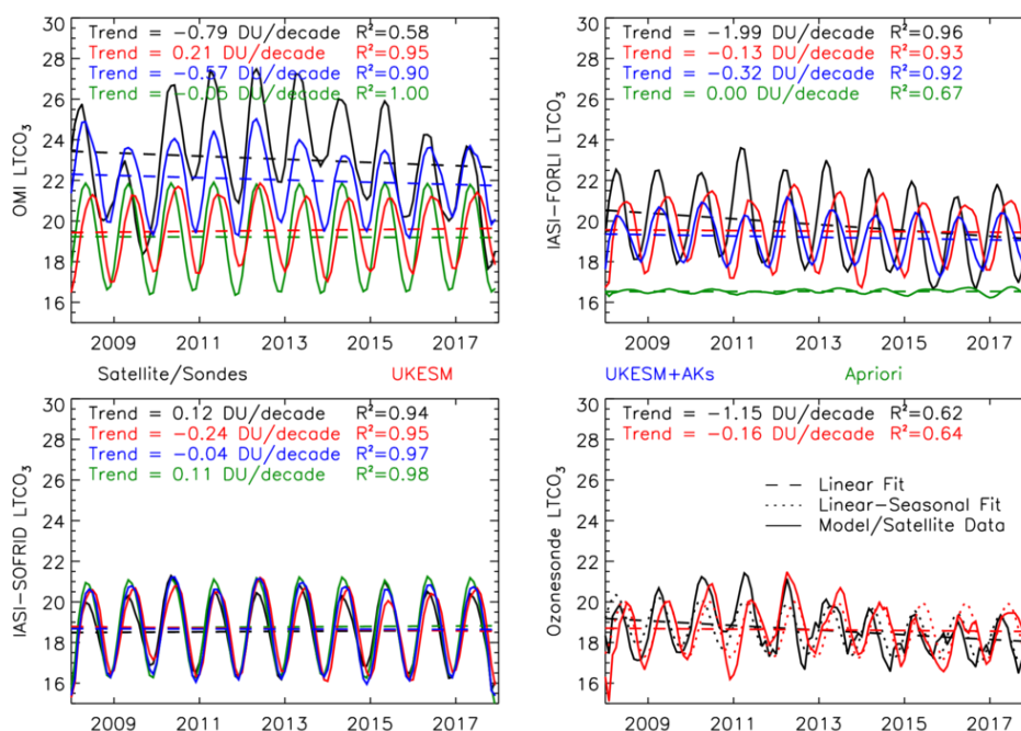
729 Figure 1: Lower tropospheric column ozone (LTCO 3 , surface to 450 hPa, DU) regional time-series for North 730 America, based on the HTAP land mask, from OMI (top-left), IASI-FORLI (top-right), IASI-SOFRID (bottom-left) 731 and ozonesondes (bottom-right) are shown by the black lines in the respective panels. UKESM simulations 732 without and with satellite averaging kernels (AKs) applied are shown in red and blue lines. Green lines show 733 the satellite apriori. Dashed lines show the LTCO 3 linear trend which are labelled in the top of each panel. The 734 R^2 squared values show the linear-seasonal trend model fit to the corresponding LTCO 3 time-series (i.e. 735 correlation squared).
