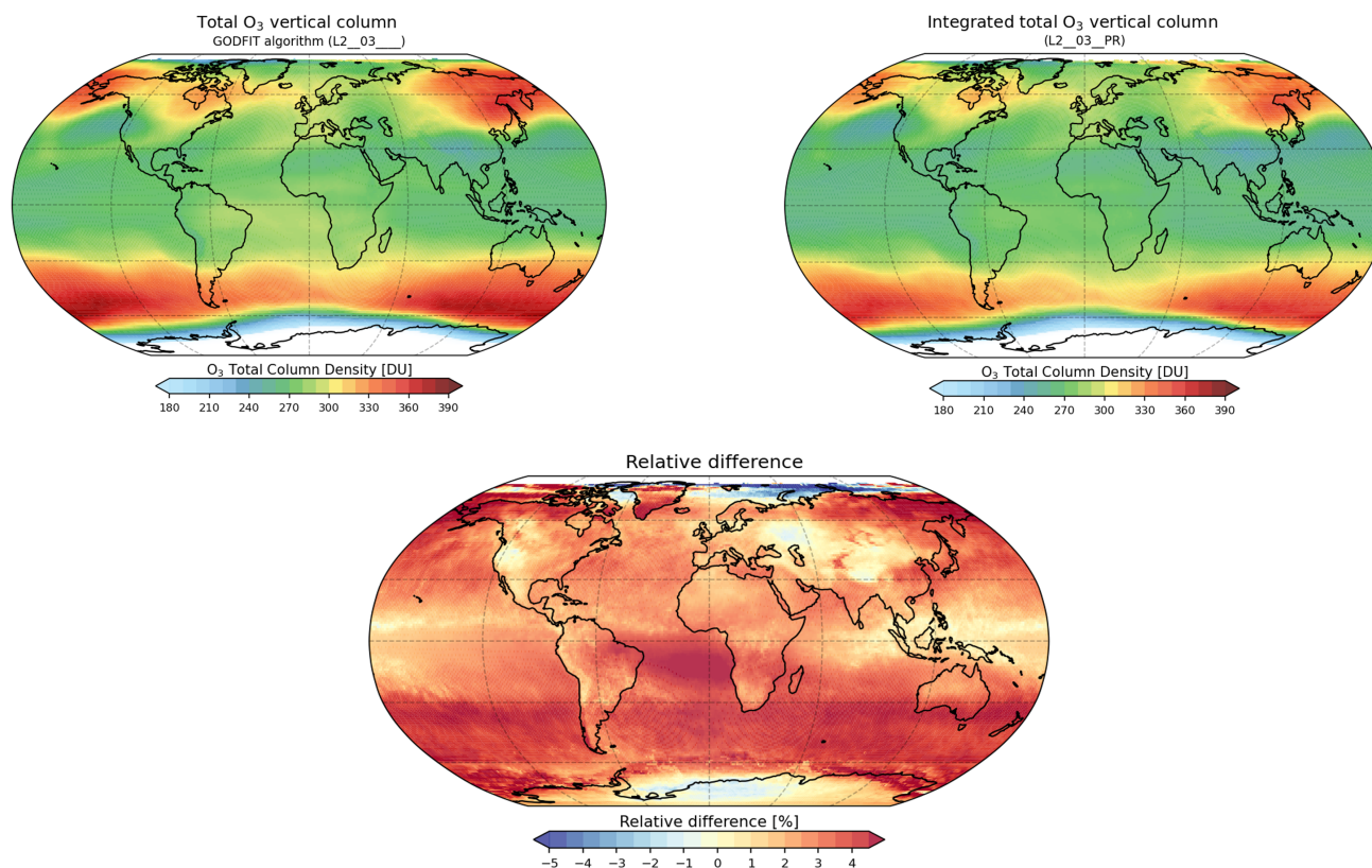
Figure 12. Relative difference (bottom) between the total ozone column of the operational TROPOMI GODFIT algorithm (L2__O3___), top left, and the integrated operational ozone profile product, top right, for October 2020.
