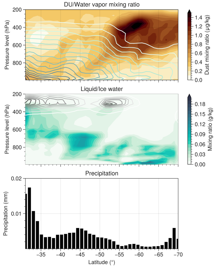
Figure A2. Vertical profiles during the 2020-02-19 Antarctic Peninsula case. Vertical profiles along the white transect in Figure 4c. Top: Dust (DU - colormap) and water vapor (contours) mixing ratio. Middle: Liquid (colormap) and ice (contours) water mixing ratio. Bottom: surface precipitation.
