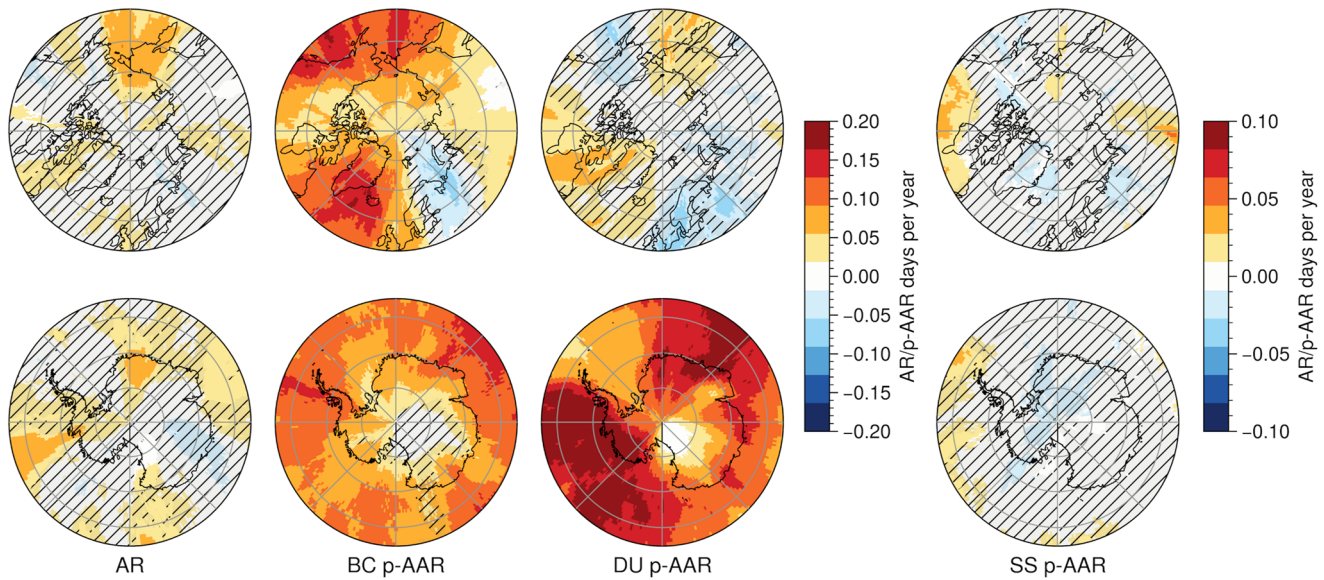
Figure 7. Trends in polar Atmospheric Rivers and polar Aerosol Atmospheric Rivers. 1980–2022 trends in Atmospheric Rivers (AR - left), Black carbon (BC - middle-left), Dust (DU - middle-right) and Sea salt (SS - right) polar Aerosol Atmospheric Rivers (p-AAR). Trend coefficients are computed as a linear regression of the time series of yearly AR/p-AAR over the period, for each grid point. Hatching indicates non-significant trends at the 95% level against a Mann-Kendall test.
