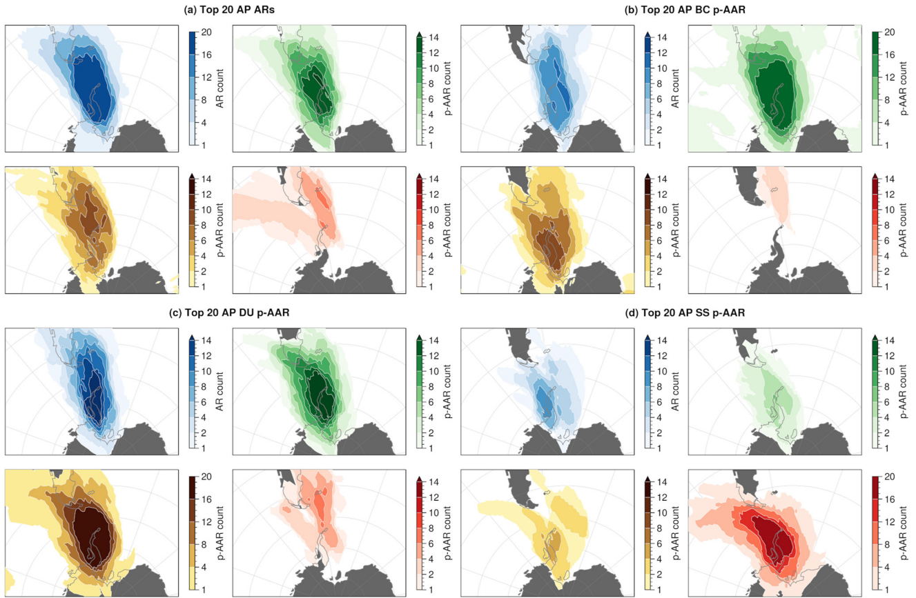
Figure A7. Top 20 Atmospheric Rivers and polar Aerosol Atmospheric Rivers in the Antarctic Peninsula. Same as Figure 10 but for Atmospheric Rivers and polar Aerosol Atmospheric Rivers reaching the Antarctic Peninsula.
