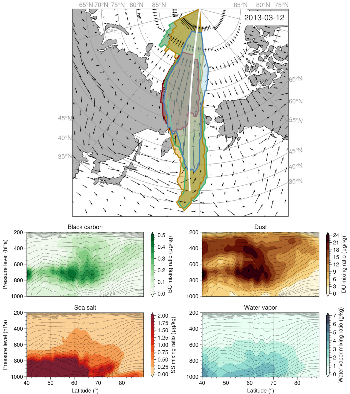
Figure 2. 2013-03-12 Asian dust transport to the high Arctic. Top: detection of Atmospheric River (AR - lightblue), Black carbon (BC - green), Dust (DU - yellow) and Sea salt (SS - red) polar Aerosol Atmospheric Rivers (p-AAR), and 500 hPa wind (arrows) on 2013-03-12. Bottom: vertical profiles of BC, DU, SS, and water vapor mixing ratio along the white transect in the top panel. Contours indicate constant levels of equivalent potential temperature (isotropes).
