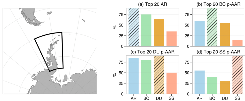
Figure 10. Top 20 polar Atmospheric Rivers and polar Aerosol Atmospheric Rivers in the Antarctic Peninsula. Same as Figure 9 but for AR/p-AAR reaching the Antarctic Peninsula (AP).
