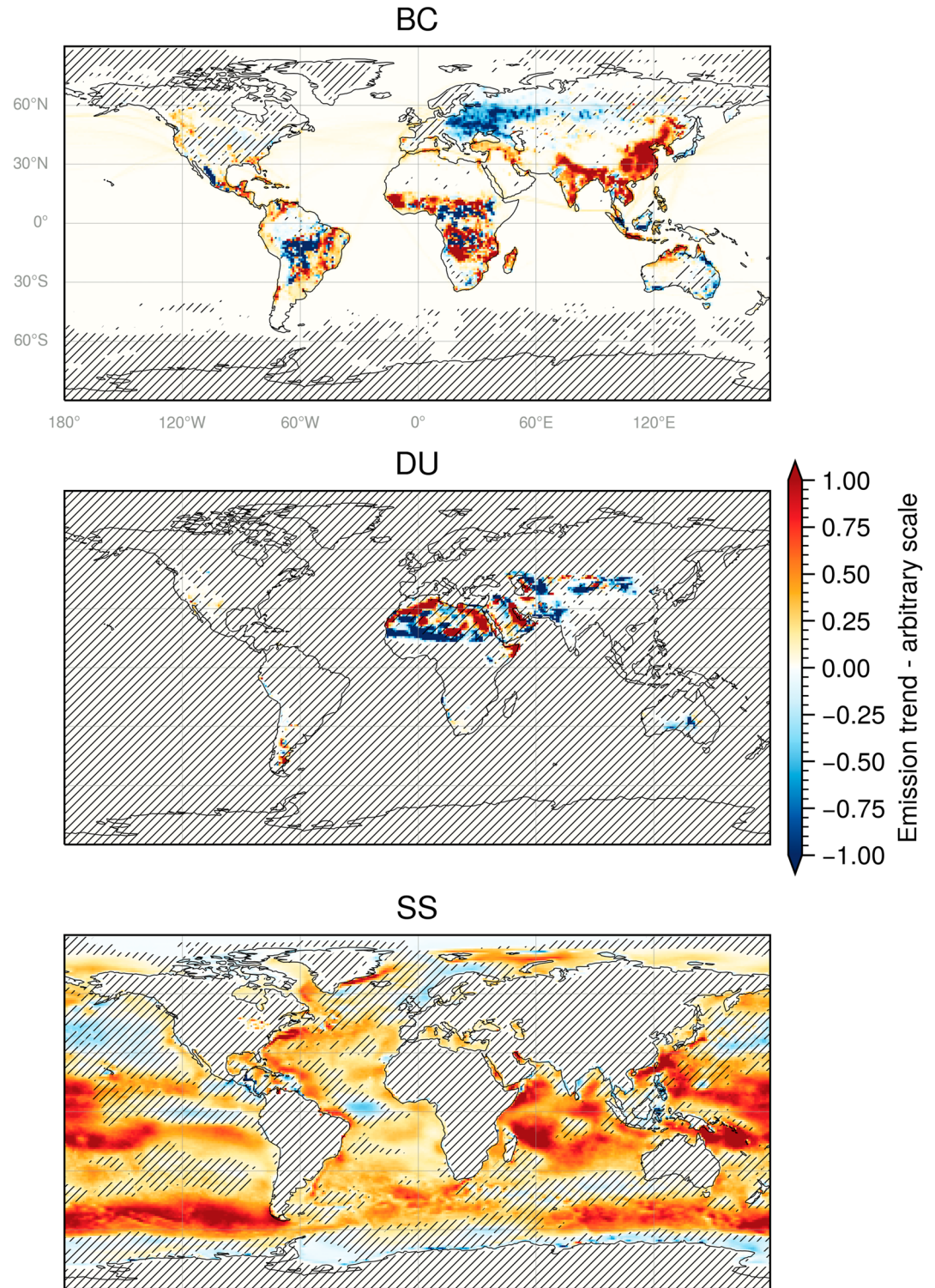
Figure A4. Aerosol emission trends. Trends in annual emissions of Black carbon (BC - top), Dust (DU - middle), Sea salt (SS - bottom) in MERRA-2 over the period 1980–2022. Hatching indicates non-significant trends at the 95% level based on a Mann-Kendall test.
