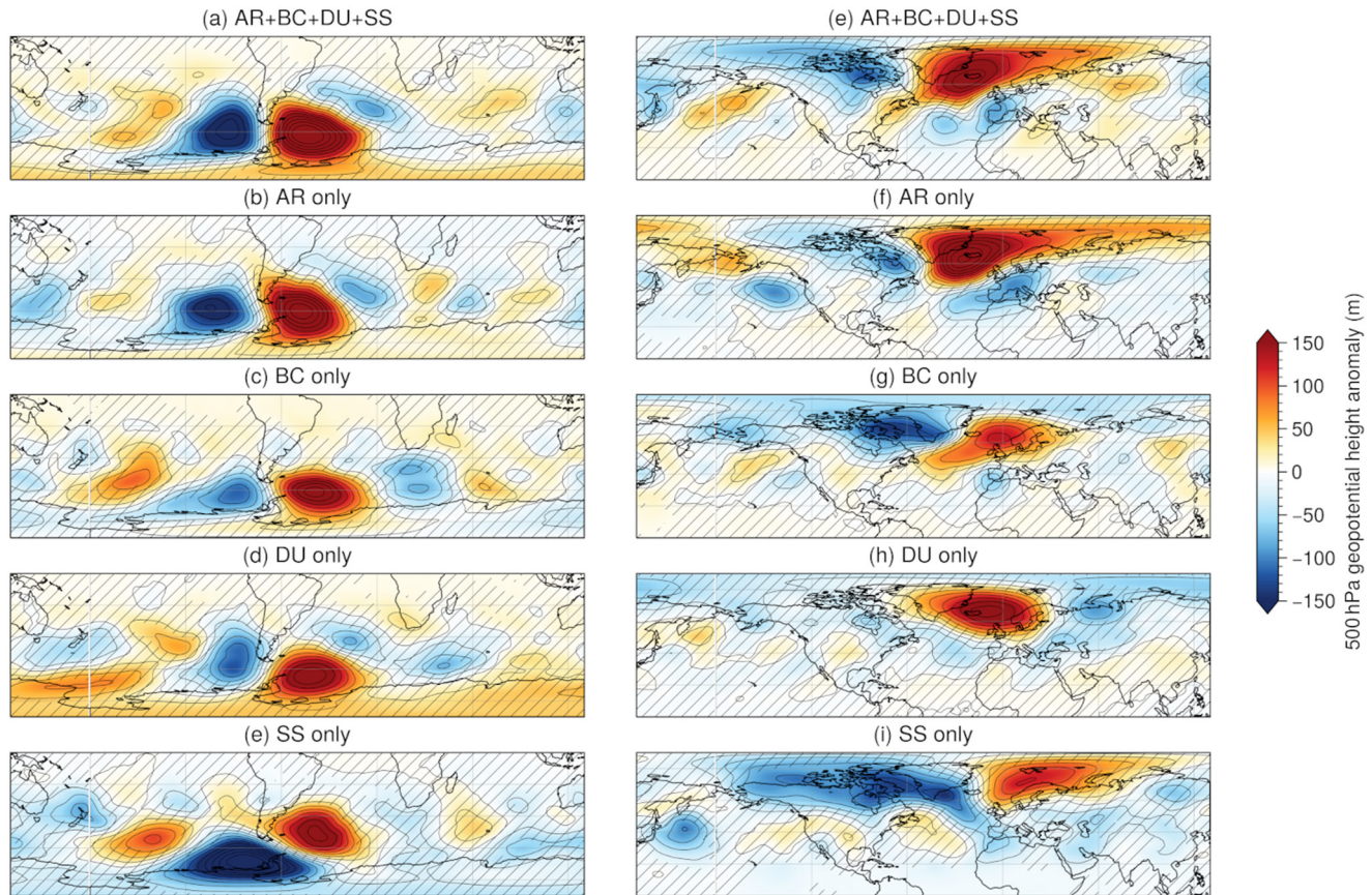
Figure 11. Geopotential height anomalies during top events. Composite of 500 hPa geopotential height anomalies for the top 20 events of 5 different types reaching the Antarctic Peninsula (left) and Greenland (right). (a, e) Co-occurring Atmospheric River (AR) and polar Aerosol Atmospheric River (p-AAR) of all aerosols. (b, f) AR only with no p-AAR. (c, g) Black carbon (BC) p-AAR only. (d, h) Dust (DU) p-AAR only. (e, i) Sea salt (SS) p-AAR only. Geopotential height from MERRA-2. Hatching indicates areas where the standard deviation of the anomaly among the events is two times larger than the absolute value of the average anomaly.
