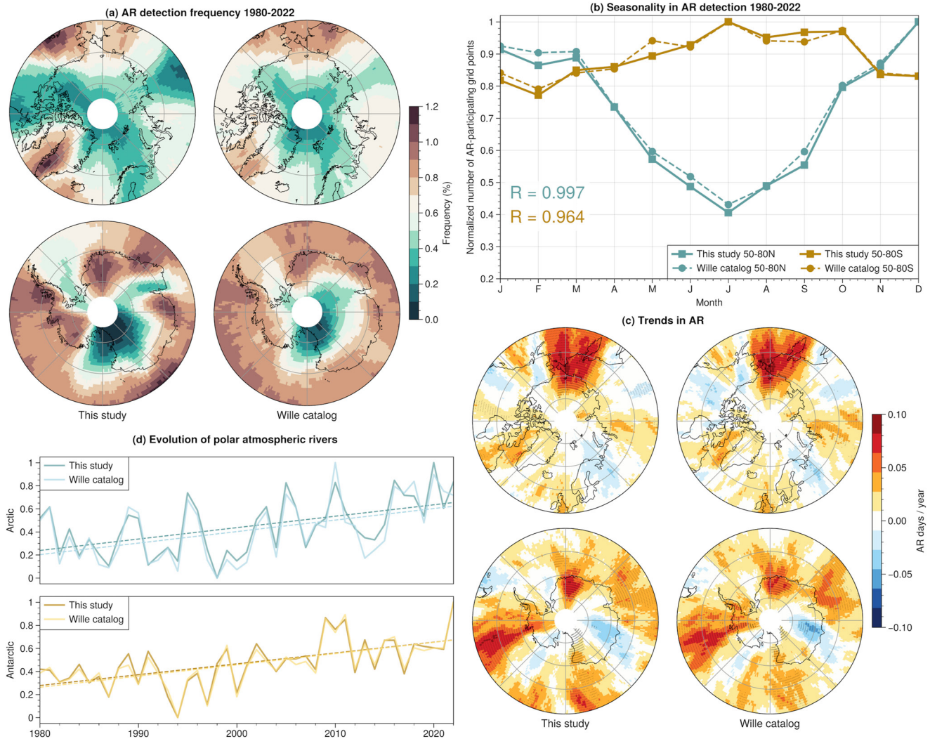
Figure A11. Validation of the adaptations made to the Wille et al. (2019) Atmospheric River detection scheme. (a) Frequency of Atmospheric River (AR) grid points detected in 1980–2022 using our method (left) and the Wille et al. (2019) method (right). (b) Seasonality in the normalized number of AR grid points above 50° N (blue) and below 50° S (gold), with our method (solid line) and the Wille et al. (2019) method (dashed line). Spatial averaging is weighted by the cell surface. R indicates the Pearson correlation coefficient between our catalog and the Wille et al. (2019) catalog. (c) Trends in AR days per year in the Antarctic, over the period 1980–2022, in this work (left) and in Wille et al. (2021) (right). (d) Relative evolution of AR frequency in the Arctic (top - 50–80° N) and Antarctic (bottom - 50–80° S) in both catalogs, for the period 1980–2022.
