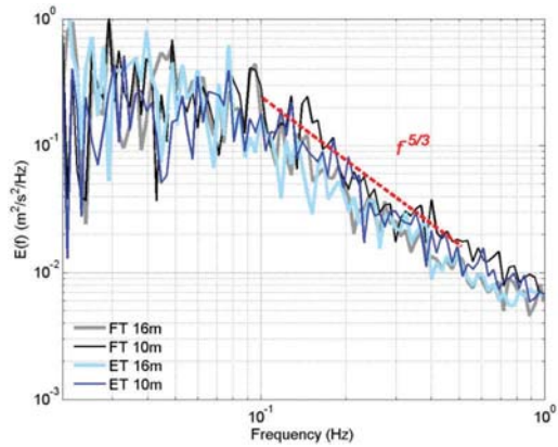
Figure 3. Power spectral density (PSD) of the current velocity (streamwise component) at depth levels 10 and 16 mab at site A on 28-Jun-2018. Velocity spectra during peak flood tide (FT) are shown by gray and black, and during ebb tide (ET) by light and dark blue. Red dashed line shows the spectral slope f^{-5/3} in the inertial subrange.
