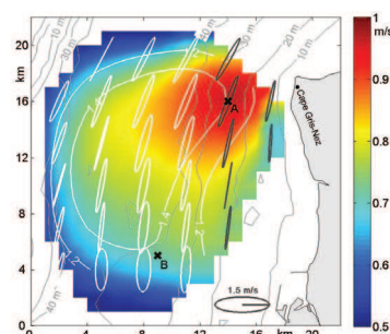
Fig. 3 Mean surface current velocity during the whole study period (color shading) and during the spring tide period in May 2003 (white contours). Shown also tidal current ellipses derived from PCA on May 16, 2003 (every third ellipse is shown). Black ellipses denote counter-clockwise rotating tidal currents and white ellipses denote clockwise rotating currents. Black crosses show locations selected for detailed analysis.
