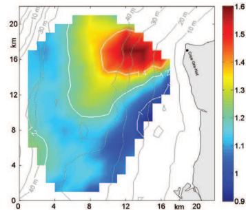
Fig. 4 Current velocity asymmetry \alpha distribution.
