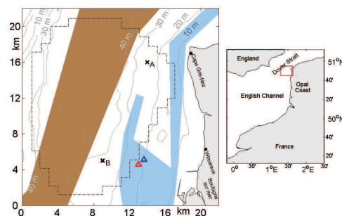
Fig. 1 Study area off the Opal coast in the eastern English Channel (red square on the right panel). Radar sites are shown by black dots and the blue and red triangles denotes the locations of ADCPs in June 2008 and July 2009 respectively. Black crosses show locations A and B selected for a detailed analysis. The navigation way of vessels travelling northward is shown by brown shading. Blue shading matches the main fishing area. Contour interval of the bathymetry is 10 m (grey solid lines). Black dashed line indicates the radar coverage zone. Geographic names used in the text are also shown.
