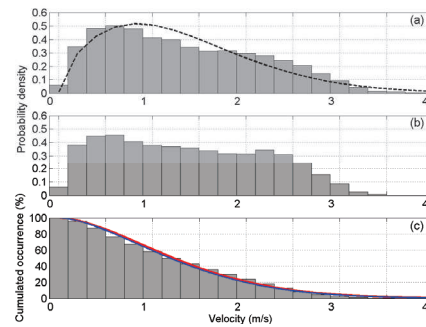
Fig. 10 Probability density in location A (a) and location B (b), and cumulated occurrence of velocity values in A (c). Weibull distribution for cumulated occurrence of velocity is shown by colour lines for A and B. Shape and scale parameters ( k and \lambda ) of Weibull law are given in the text. Dashed line in (a) represents Weibull approximation of velocity probability density.
