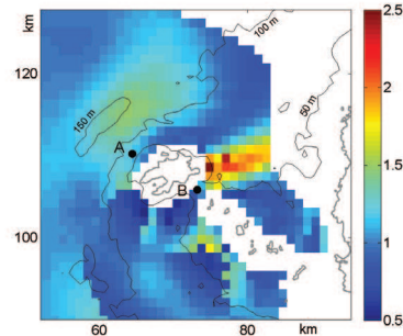
Fig. 9 Spatial distribution of current velocity asymmetry \alpha .
