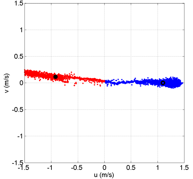
Fig. 3. Tidal current ellipse derived from ADV measurements. Red and blue points represent velocity of flood and ebb flow respectively. Full and empty circles indicate the time average flood and ebb flow velocity values.
